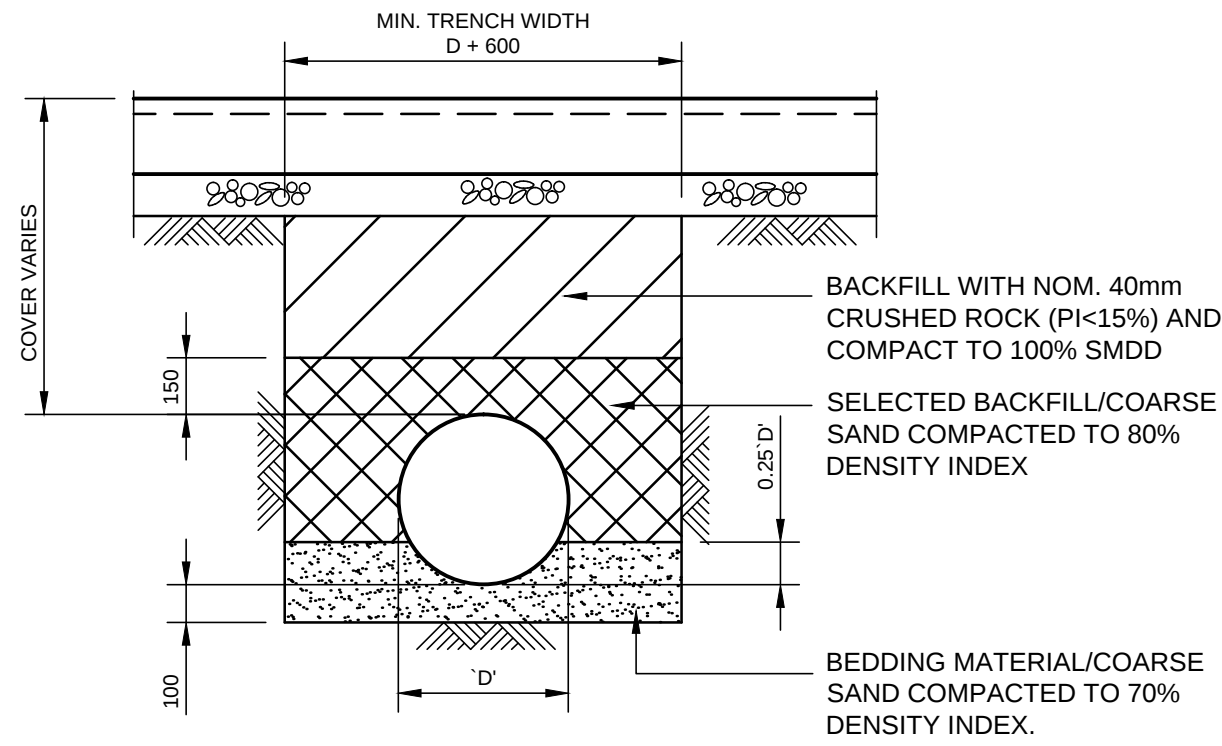
TYPICAL PIPE TRENCH DETAIL
