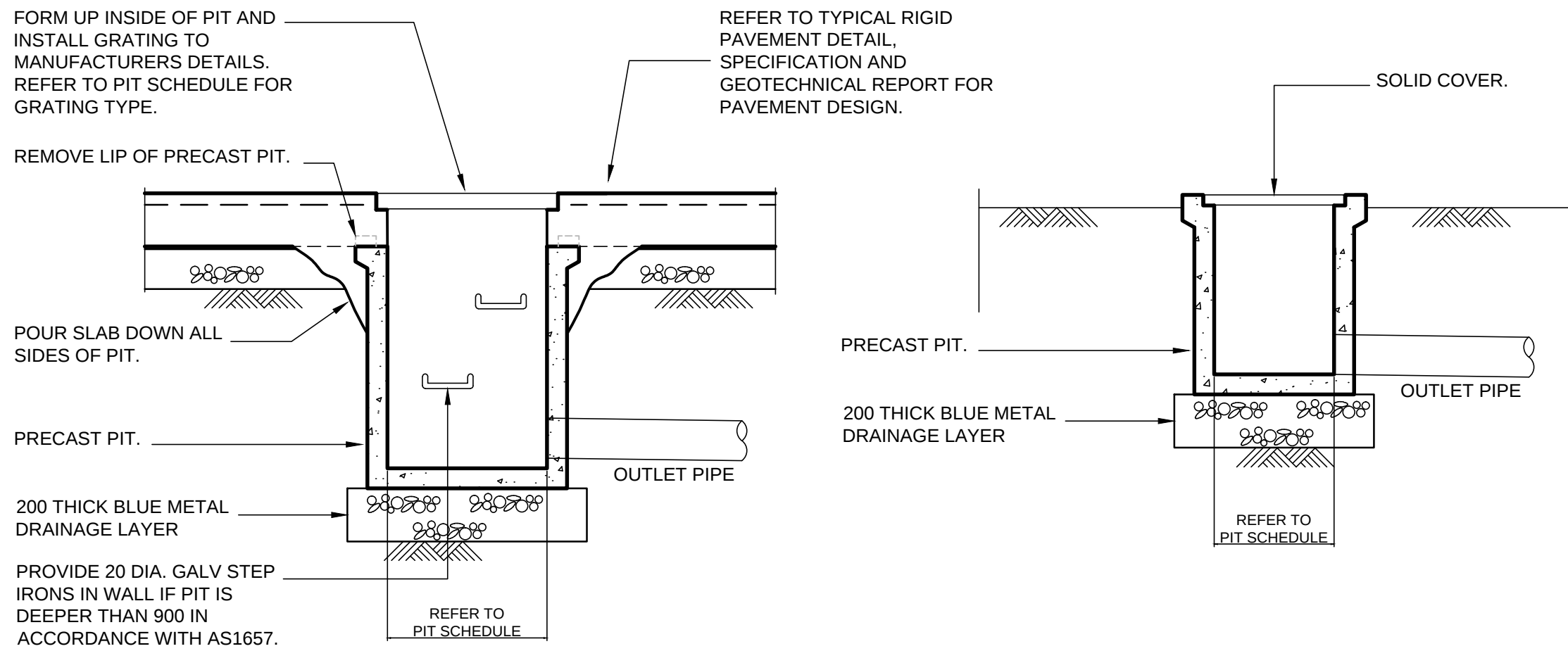
TYPICAL PRECAST STORMWATER DRAINAGE PIT DETAILS
