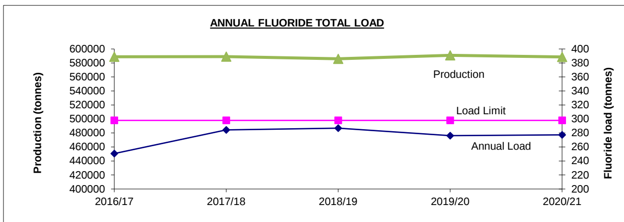
Figure 4.2B: ANNUAL FLUORIDE TOTAL LOAD FOR THE TOMAGO ALUMINIUM SMELTER (2016/17 – 2020/21)
