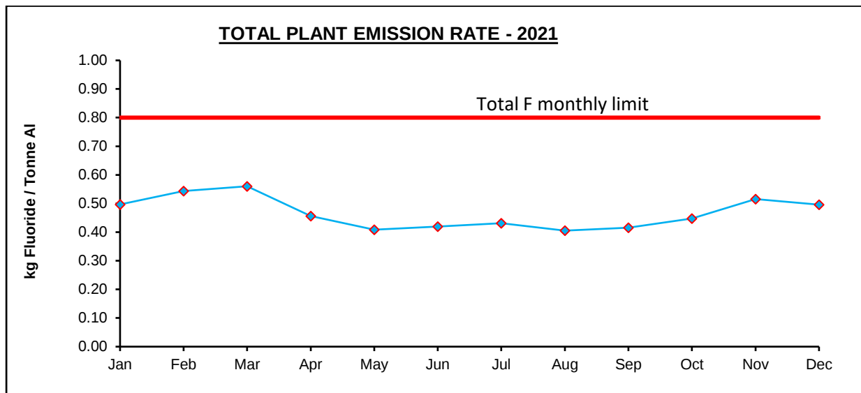
Figure 4.1: TOTAL MONTHLY FLUORIDE EMISSION RATES FROM THE TOMAGO ALUMINIUM SMELTER
