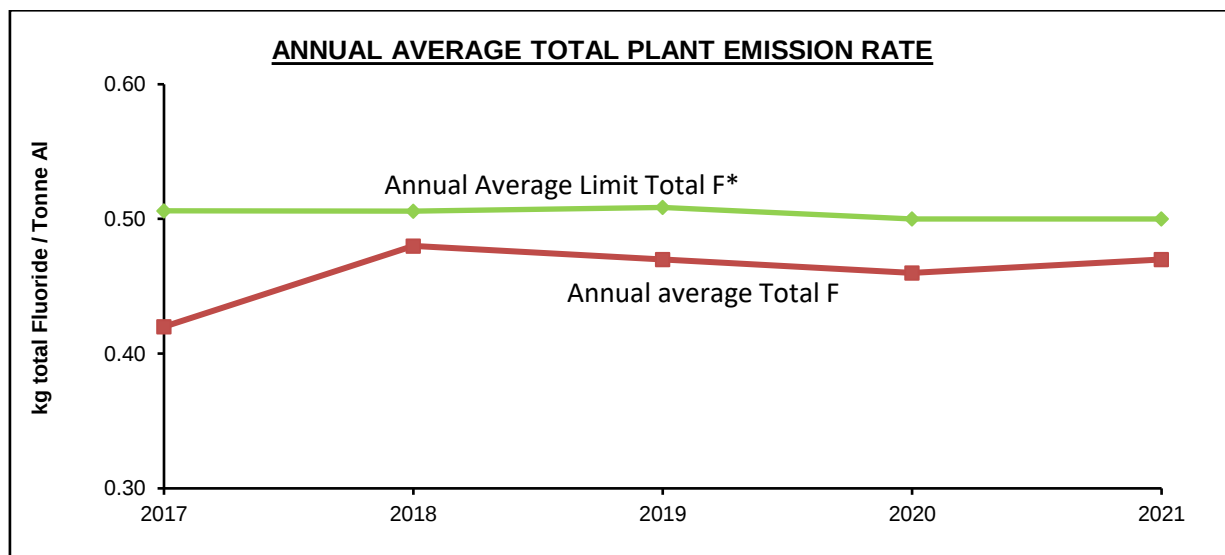
Figure 4.2A: ANNUAL AVERAGE FLUORIDE EMISSION RATES FOR THE TOMAGO ALUMINIUM SMELTER (2017 - 2021)
