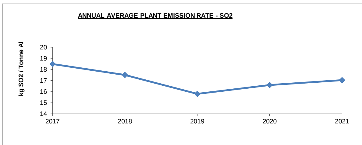
Figure 4.4: ANNUAL SULFUR DIOXIDE EMISSION RATES FOR THE TOMAGO ALUMINIUM SMELTER (2017 – 2021)
