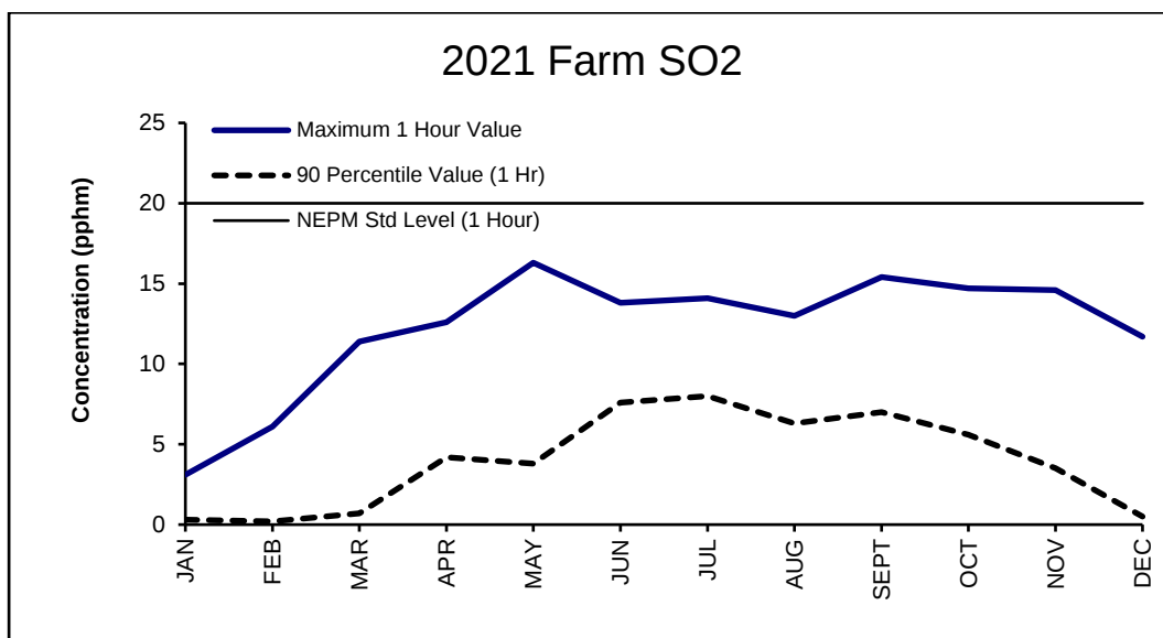
Figure 4.8B: SULFUR DIOXIDE CONCENTRATIONS IN AMBIENT AIR FOR 2021 COMPARED TO 1 HOUR ASSESSMENT CRITERIA (Farm)
