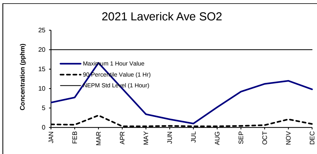
Figure 4.8D: SULFUR DIOXIDE CONCENTRATIONS IN AMBIENT AIR FOR 2021 COMPARED TO 1 HOUR ASSESSMENT CRITERIA (Laverick Ave)
