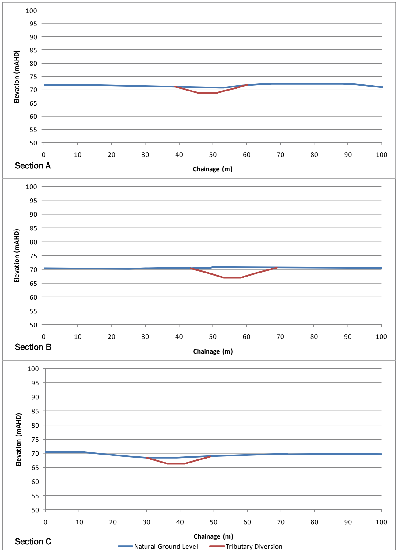
Figure 3.5 Unnamed Tributary Diversion Cross Sections
