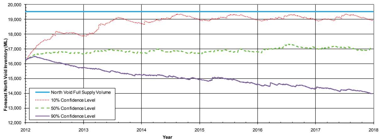
Figure 4.3 North Void Forecast Assessment
