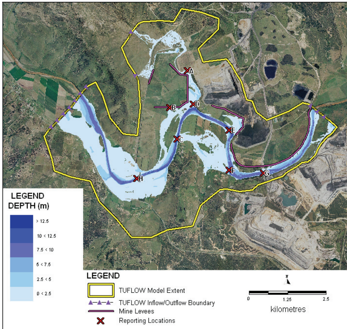
Figure 5.5 Stage 1 Levees Q10 Flood Depths
