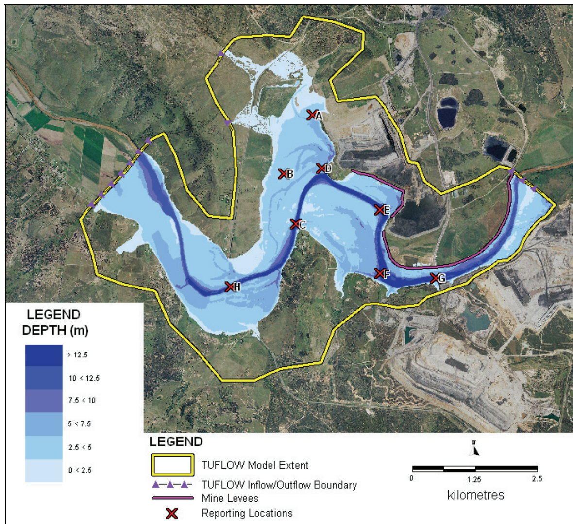
Figure 5.2 Existing Conditions and End of Mine Q100 Flood Depths
