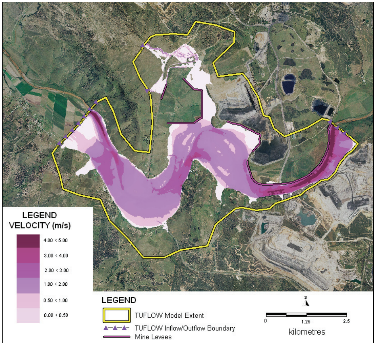
Figure 5.8 Stage 1 Levees Q100 Flood Velocities
