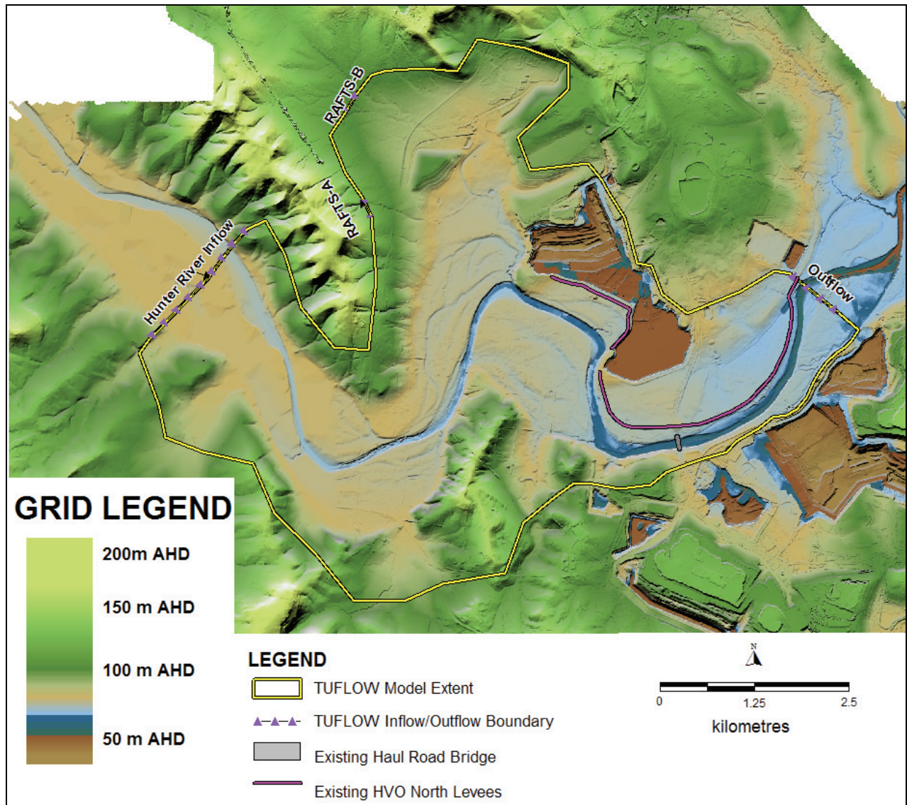
Figure B.7.7 Existing TUFLOW Model Configuration
