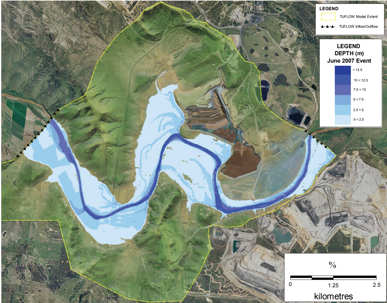
Figure B.7.9 Modelled Flood Depth June 2007 Event
