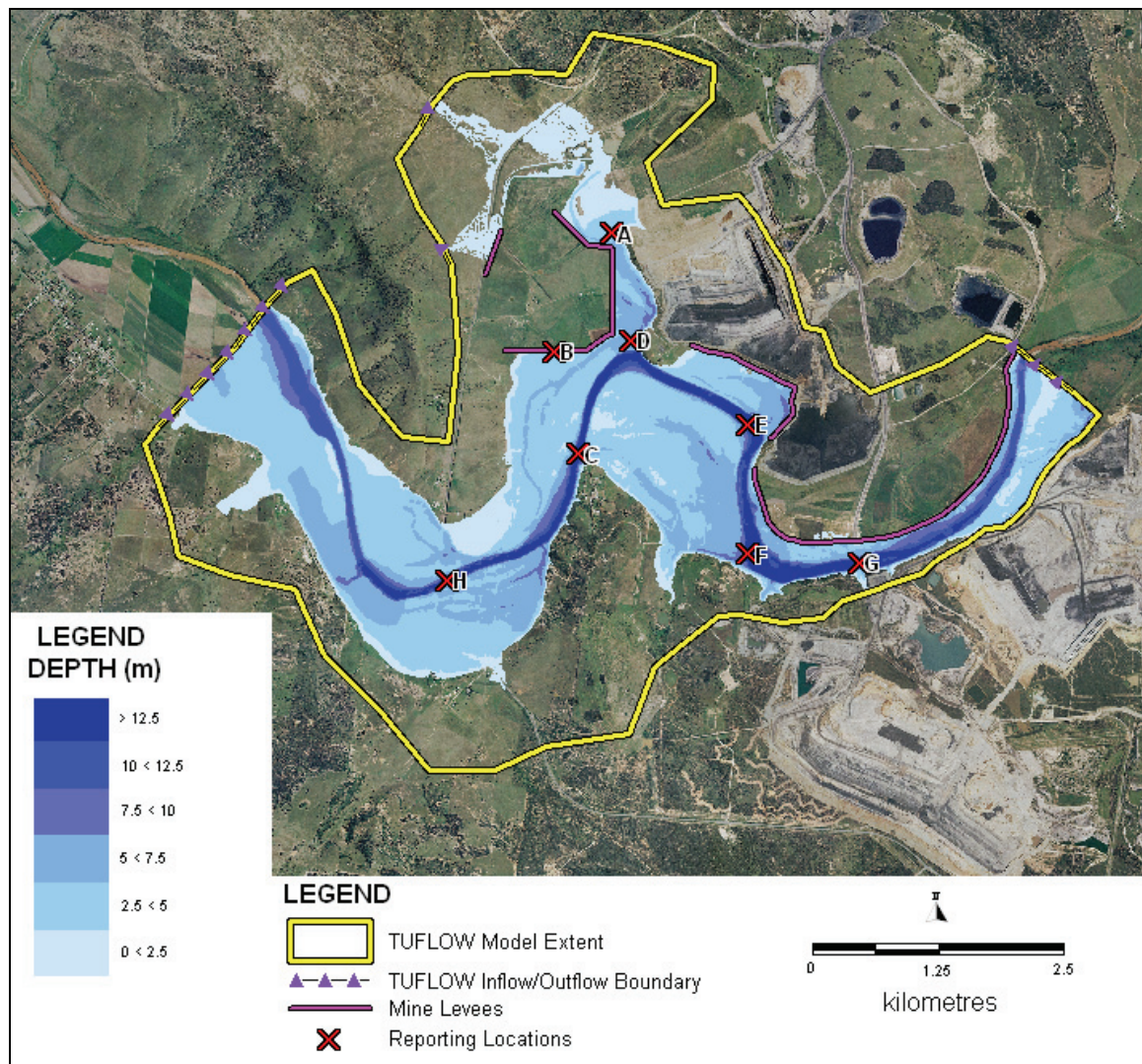
Figure 5.6 Stage 1 Levees Q100 Flood Depths
