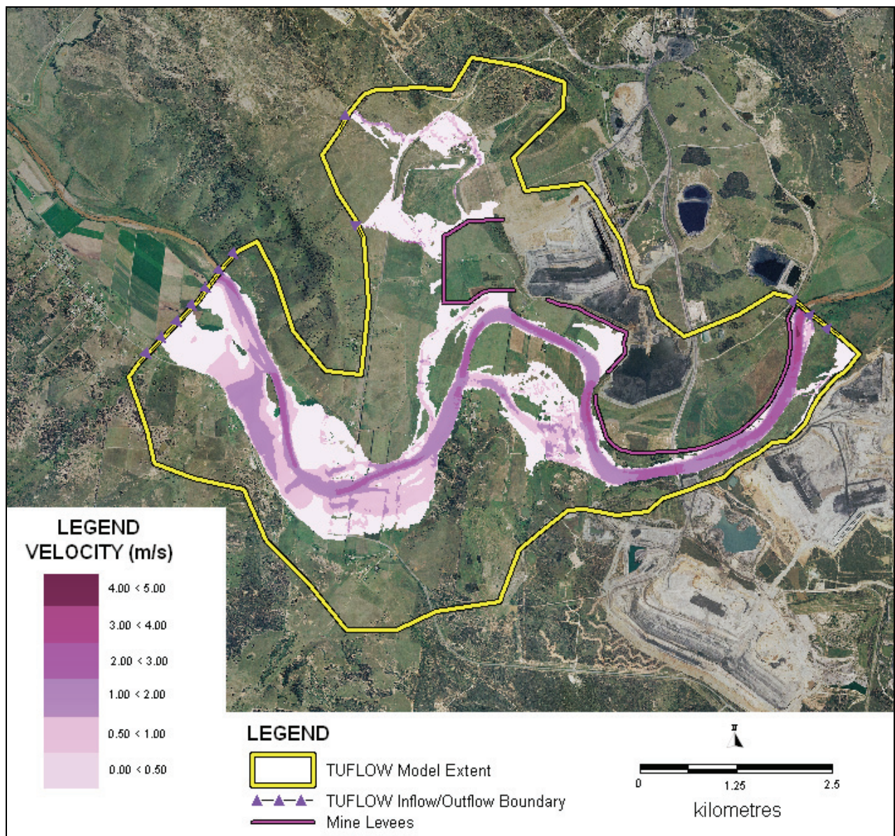
Figure 5.13 Stage 2 Levees and Channel Q10 Flood Depths
