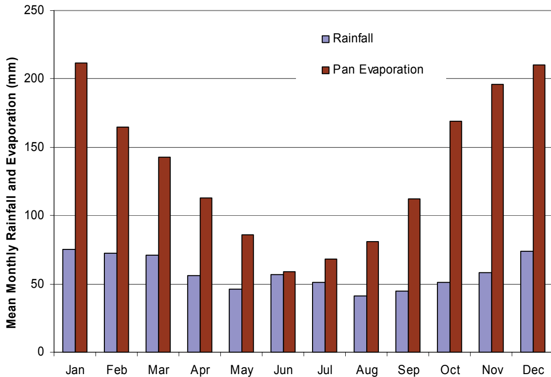
Figure 2.3 Distribution of Monthly Rainfall (Singleton Post Office) and Evaporation (Jerrys Plains Post Office)
