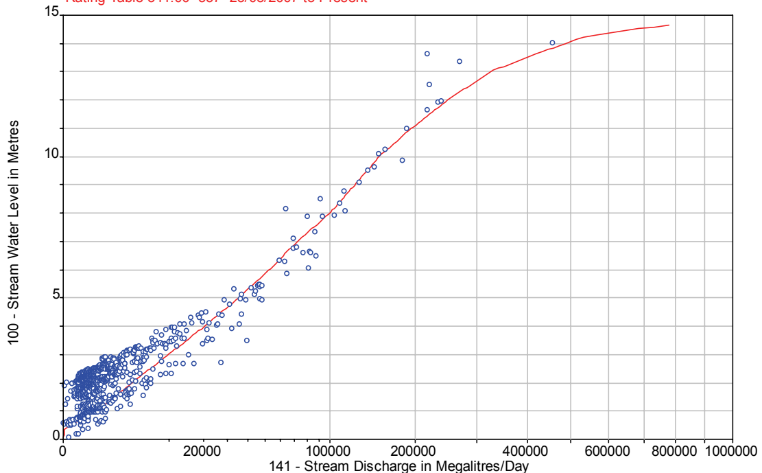
Figure B.7.2 Available Rating Curve, Hunter River at Singleton (210001)
