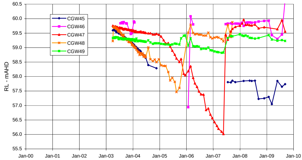
Piezometers CGW45, 46, 47, 48, 49 - alluvium
