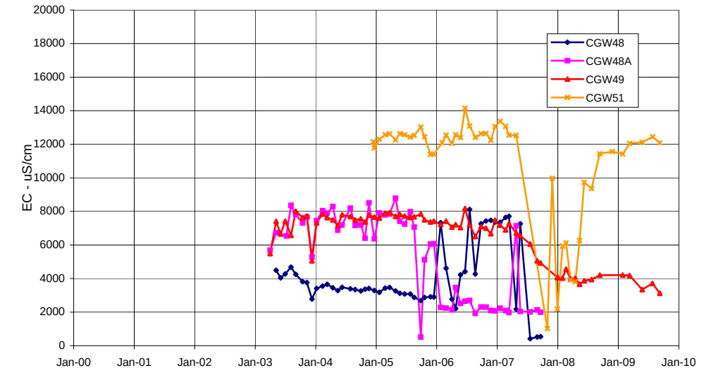
Carrington - EC at piezometers CGW48, 48A, 49, 51
