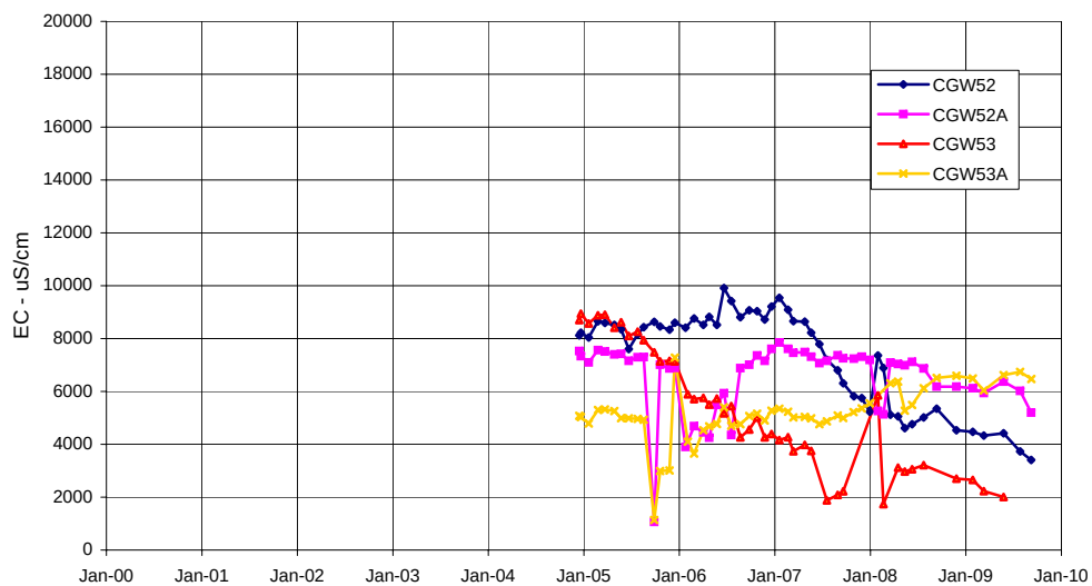
EC at piezometers CGW52, 52A, 53, 53A
