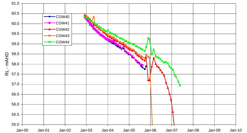
Piezometers CGW 40, 41, 42, 43, 44 - alluvium
