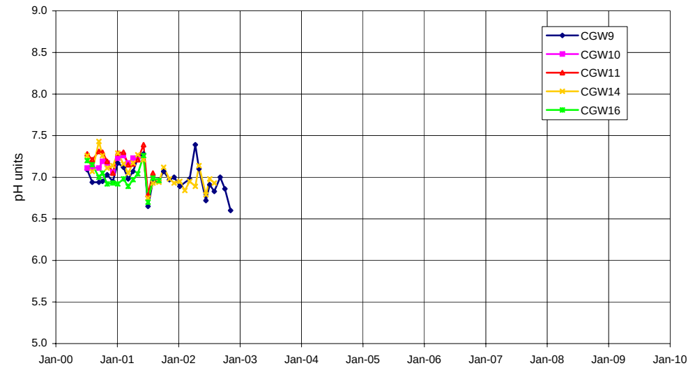
pH at piezometers CGW9, 10, 11, 14,16
