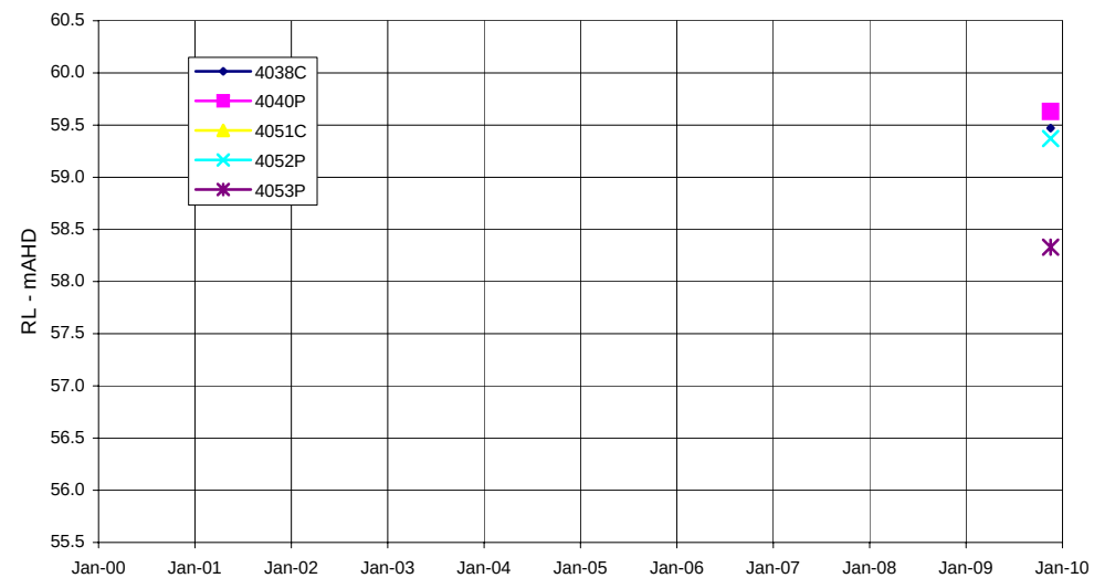
Piezometers 4038C, 4040P, 4051C, 4052P, 4053C - alluvium
