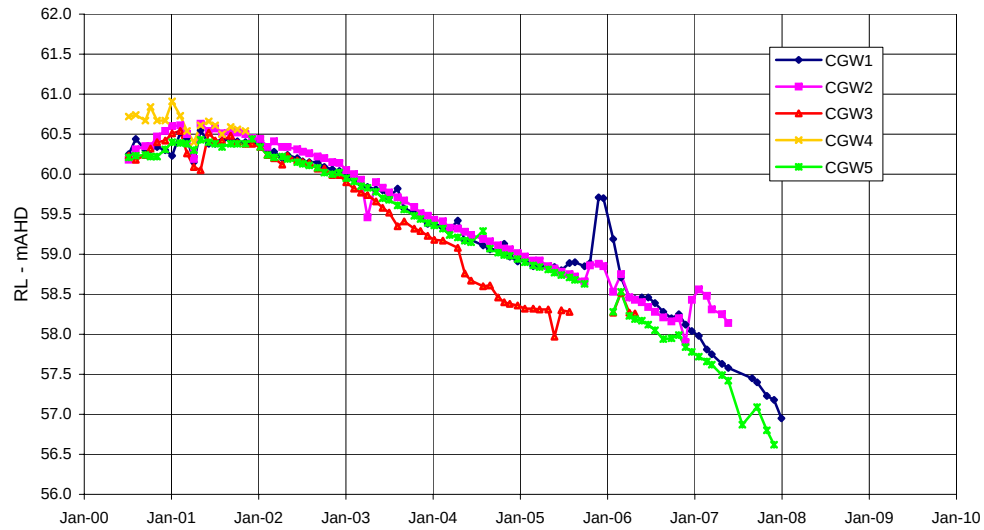
Piezometers CGW1, 2, 3, 4, 5 - alluvium
