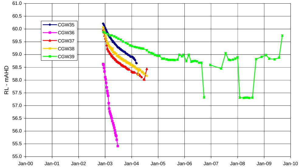
Piezometers CGW 35, 36, 37, 38, 39 - alluvium
