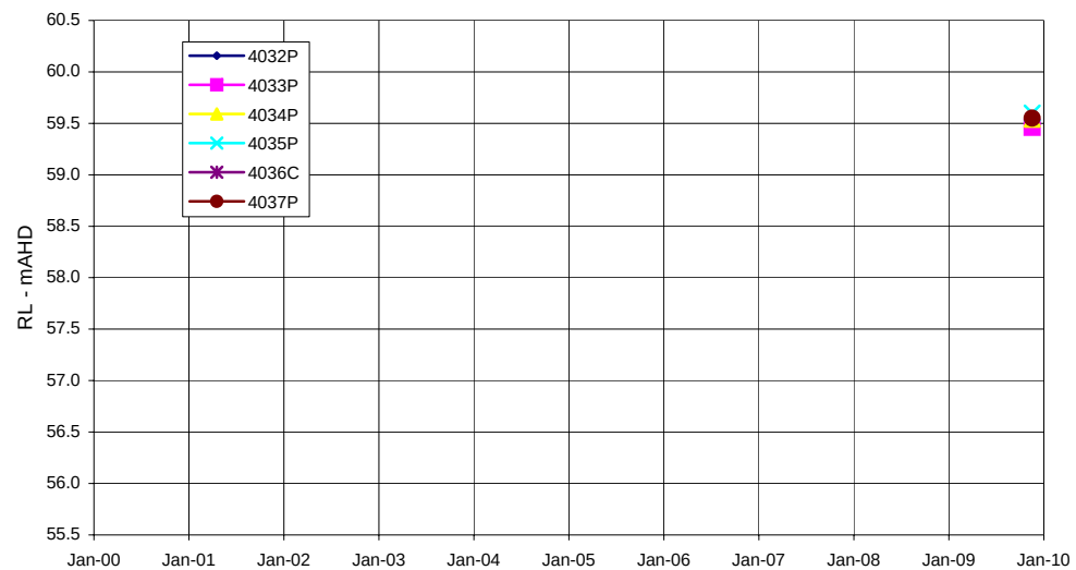
Piezometers 4032P, 4033P, 4034P, 4035P, 4036C, 4037P - alluvium
