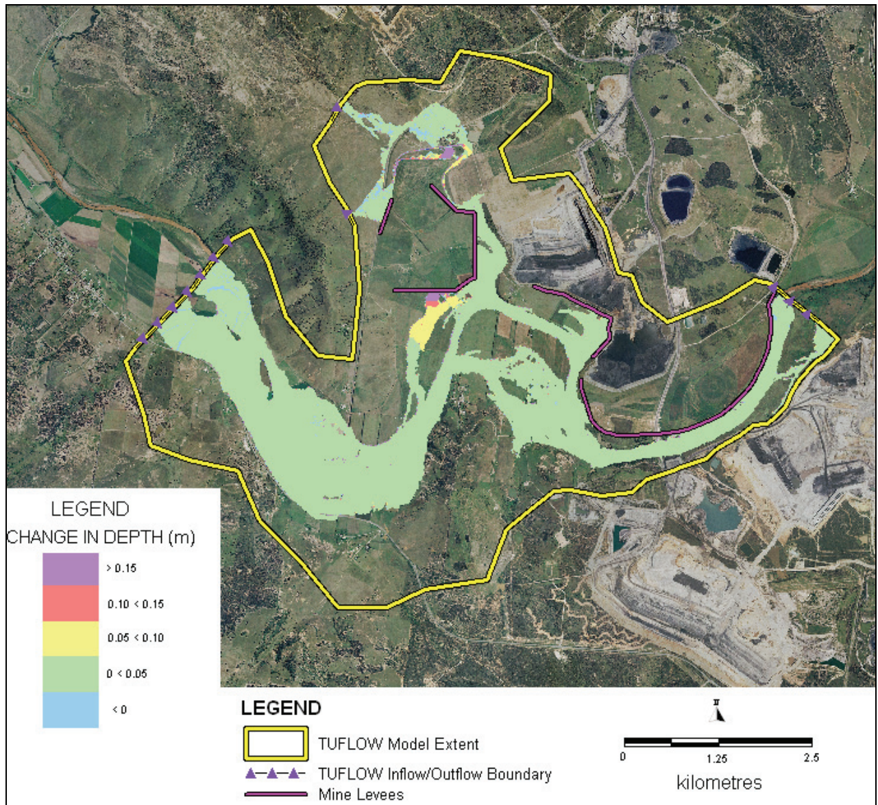
Figure 5.9 Stage 1 Levees Q10 Flood Level Impacts (compared to existing case)
