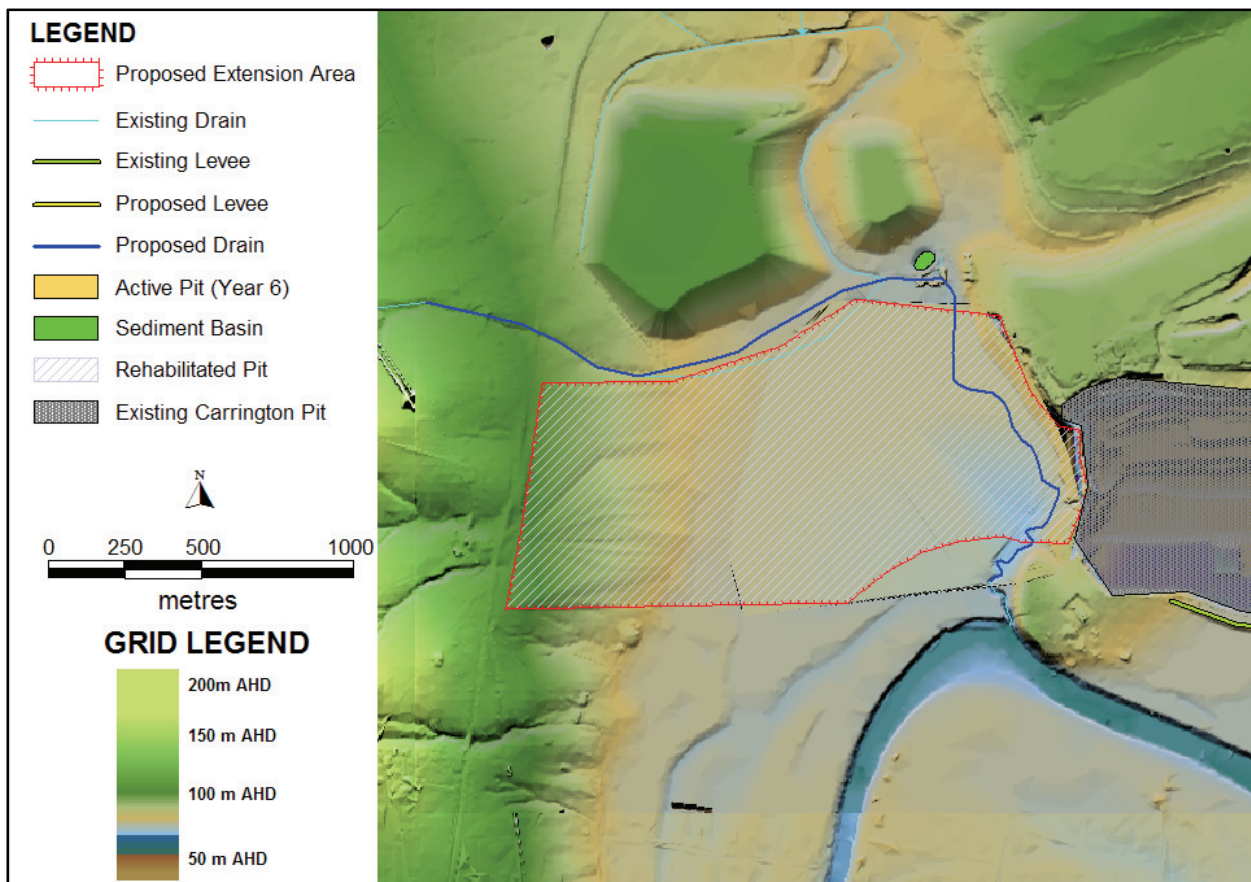
Figure 3.3 End of Mine Levees and Drainage Channels
