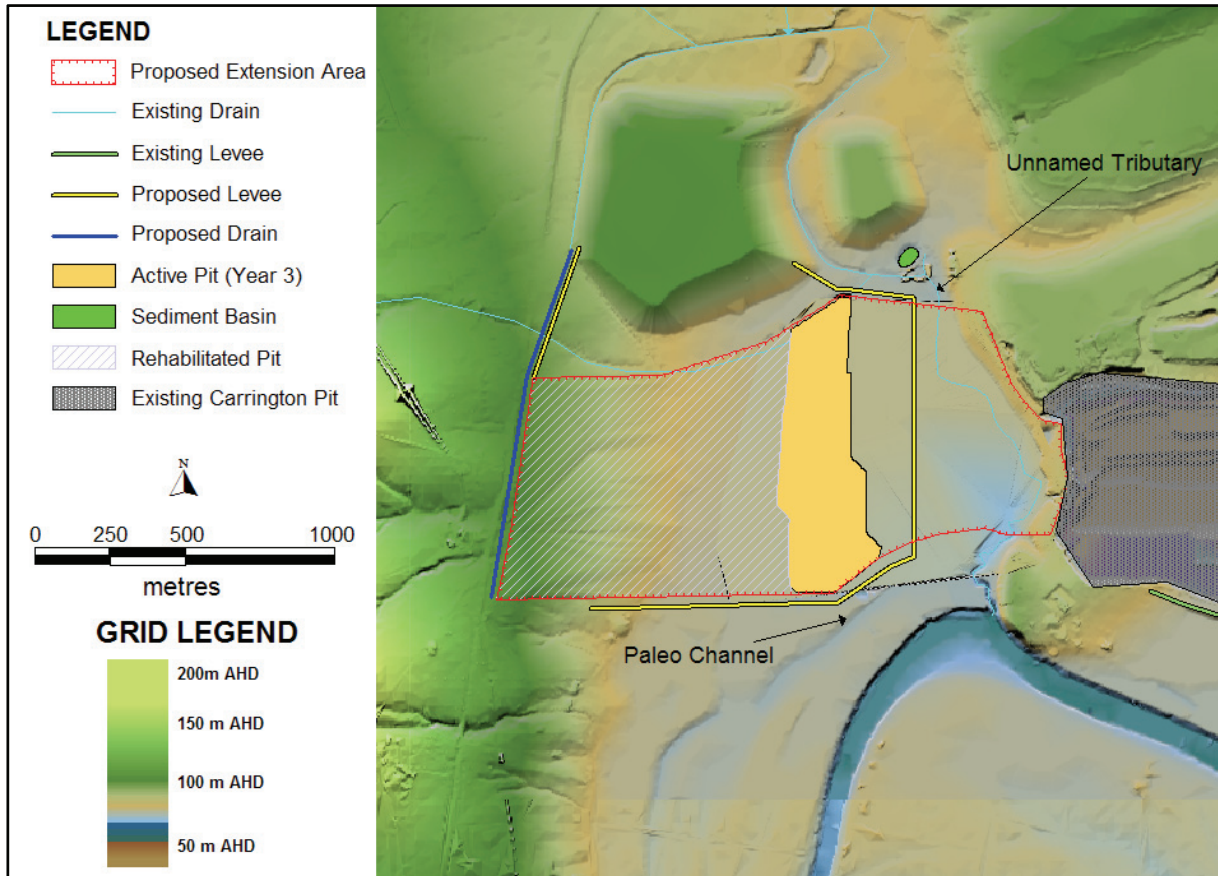
Figure 3.1 Stage 1 Levees and Drainage Channels
