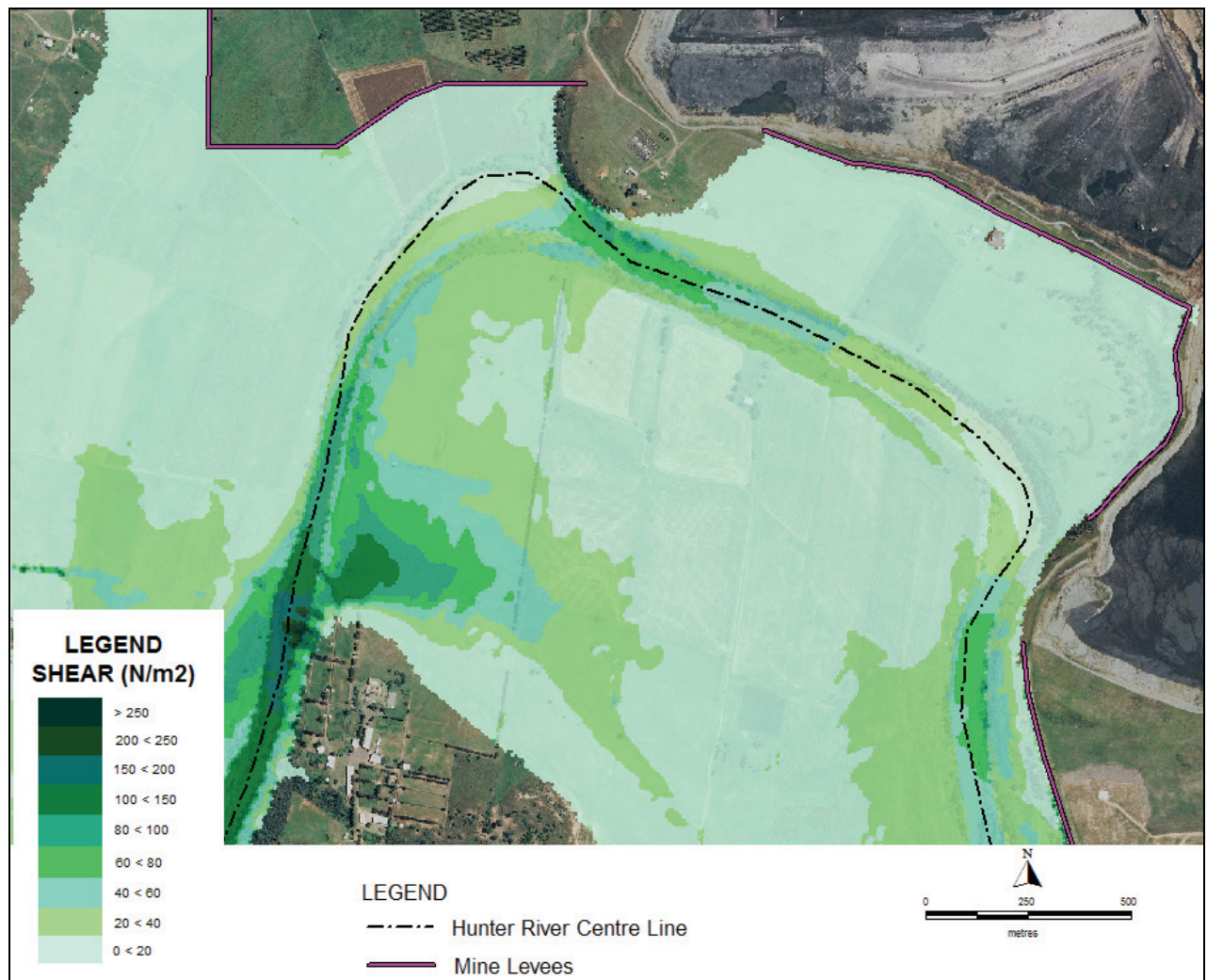
Figure 5.19 Hunter River Bed Shear , 100 Year ARI Flood
