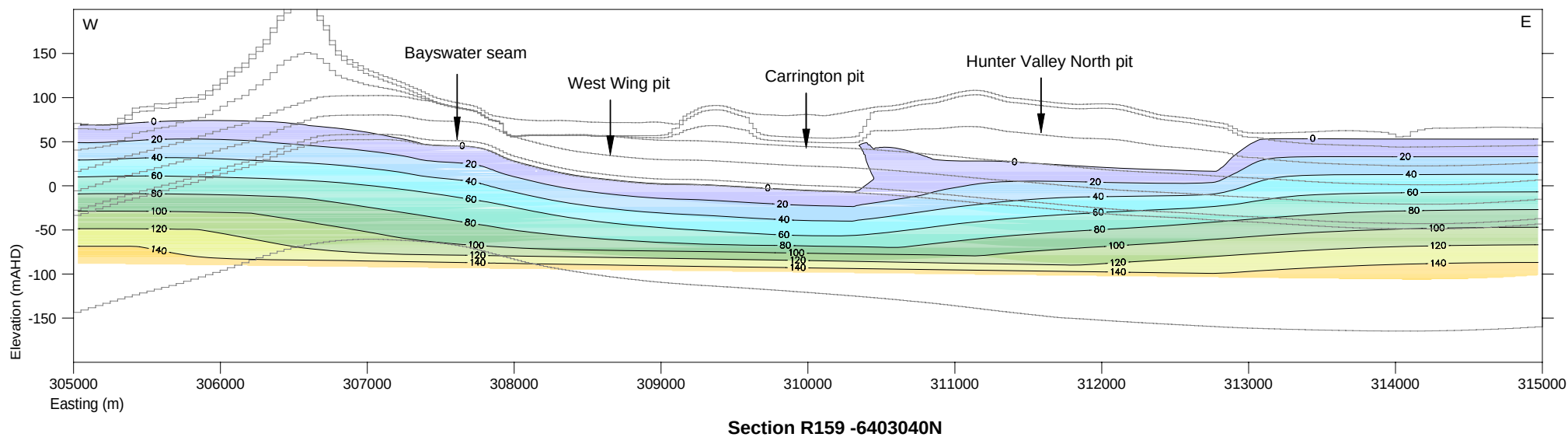
Pore pressures at vertical sections R159 and C103 at the end of mining
