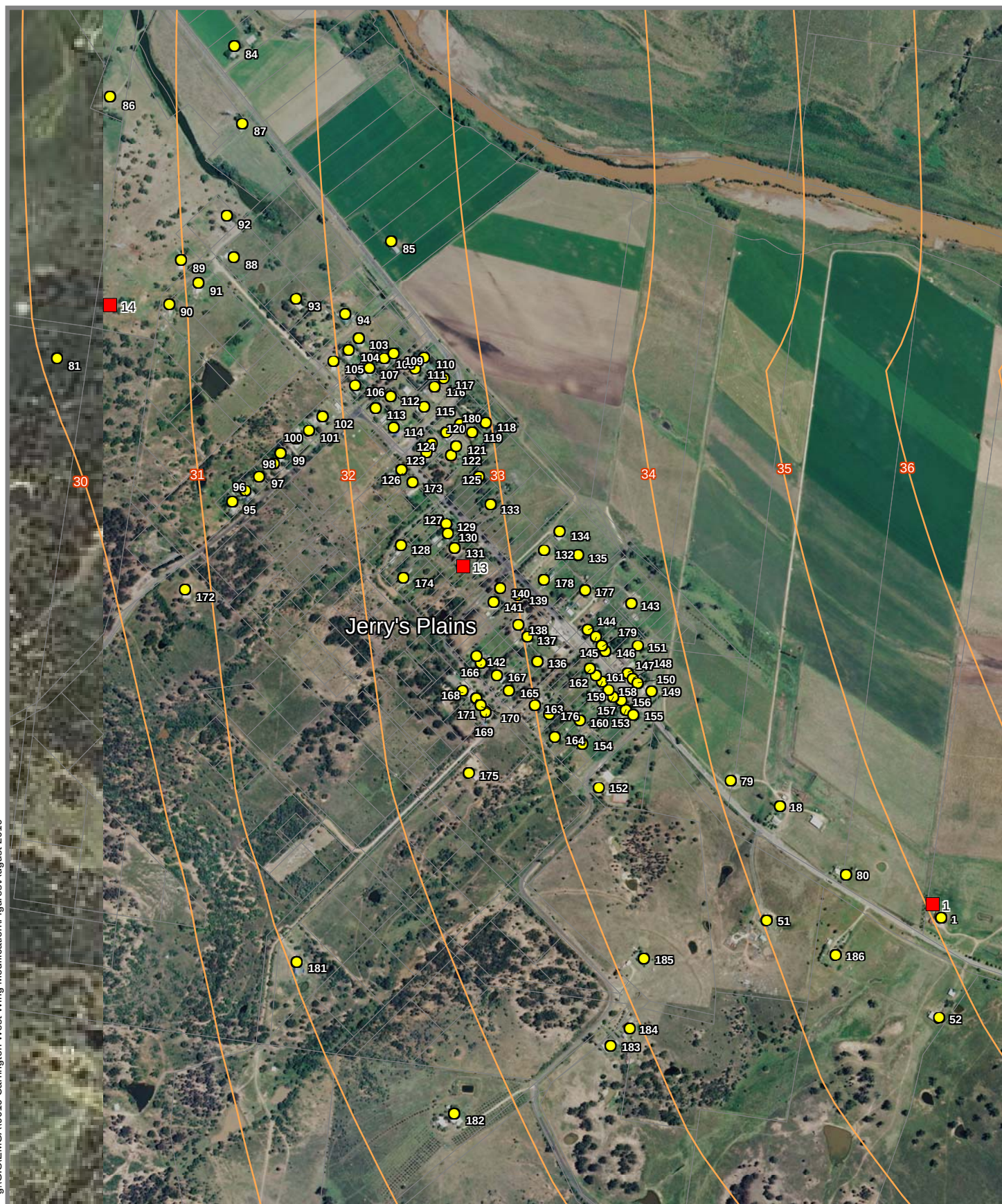
Figure 3.3a Year 5 Mitigated INP Weather Noise Levels (CWW Only) For Jerrys Plains Area
