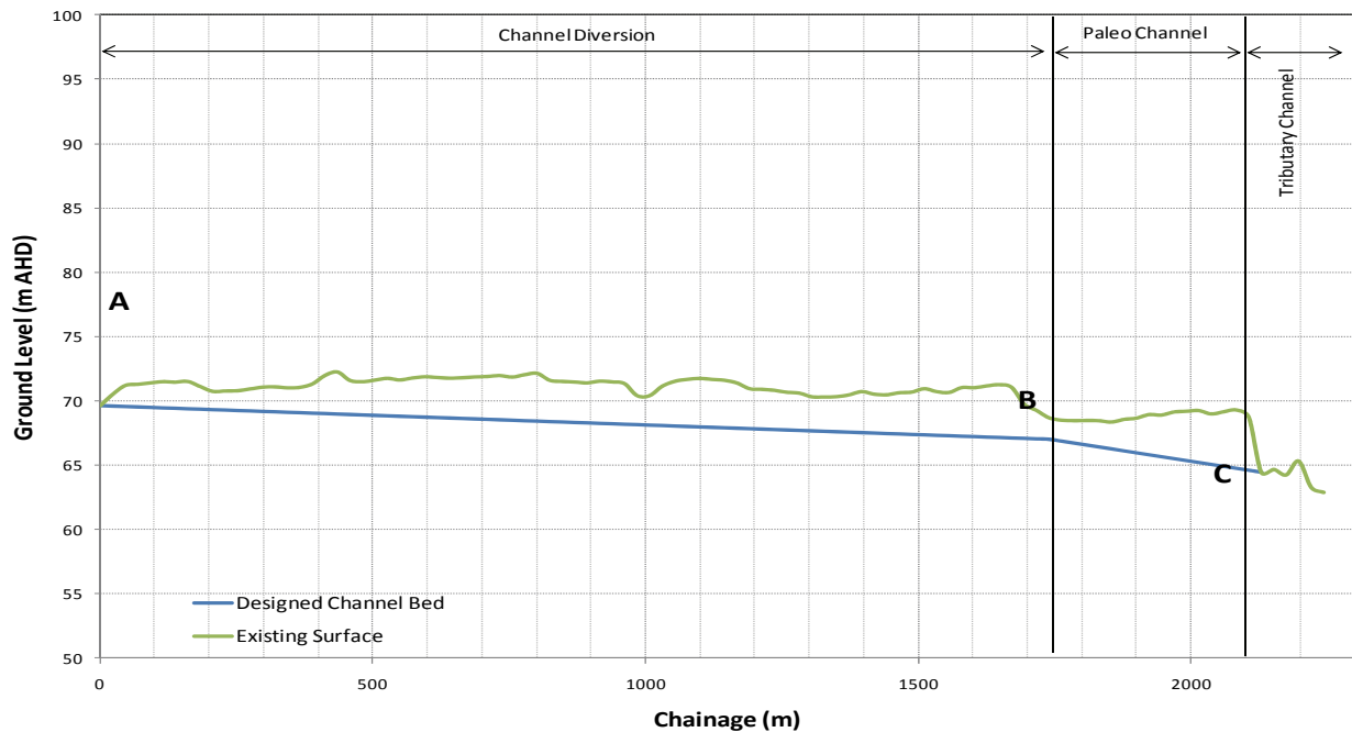
Figure 3.6 Unnamed Tributary Diversion Longitudinal Section Profile
