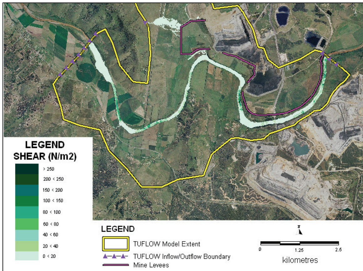
Figure 5.17 Hunter River Bed Shear, 2 Year ARI Flood
