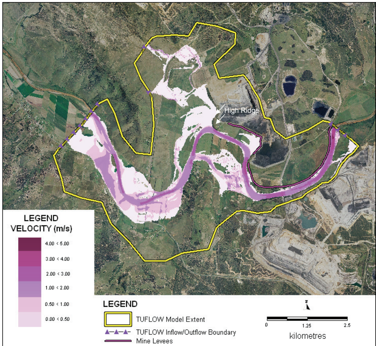
Figure 5.3 Existing Case and End of Mine Q10 Flood Velocities
