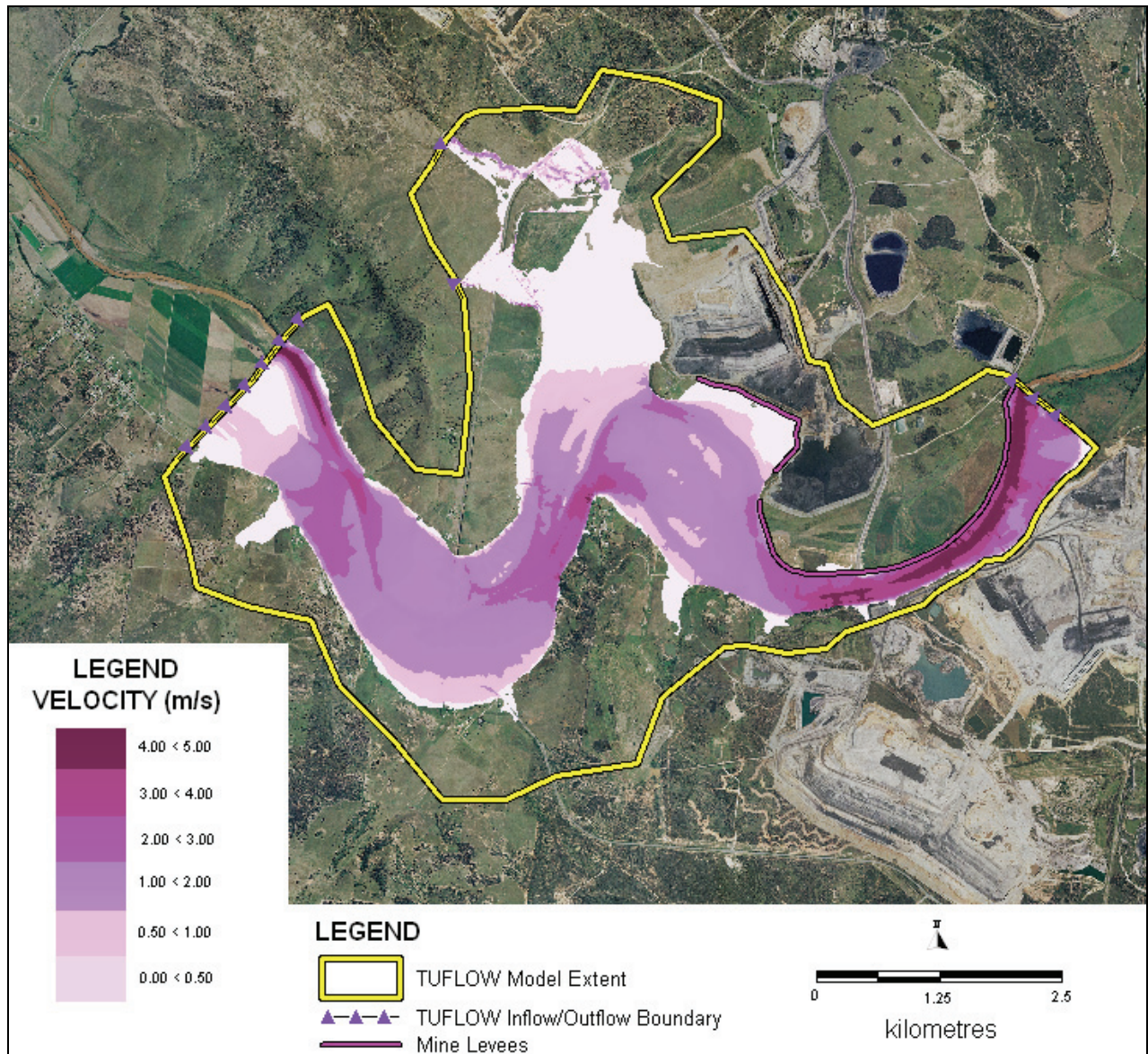
Figure 5.4 Existing Case and End of Mine Q100 Flood Velocities
