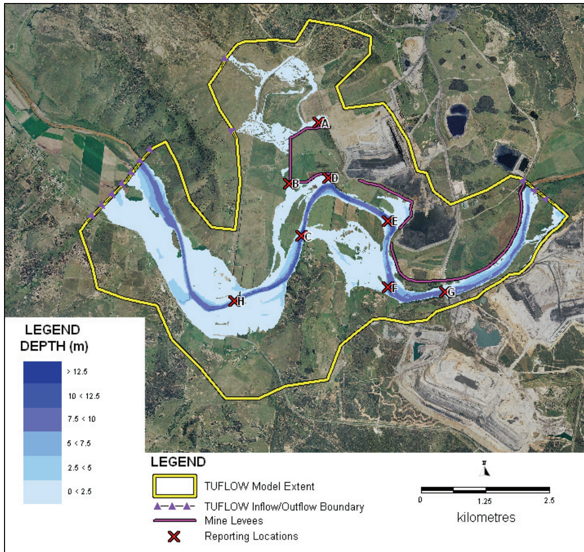
Figure 5.11 Stage 2 Levees and Channel Q10 Flood Depths
