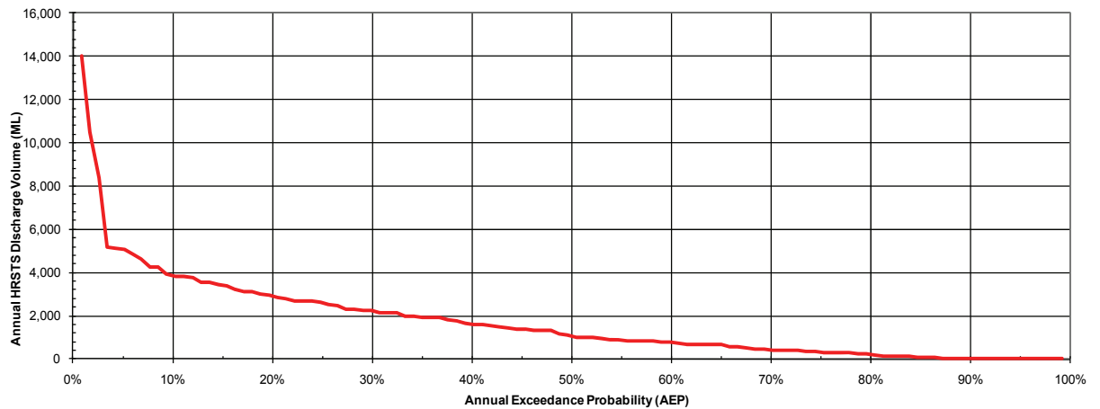
Figure 4.4 HRSTS Discharge Assessment
