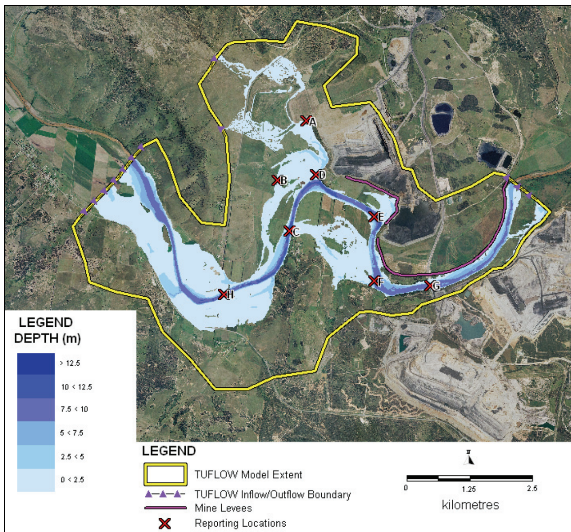
Figure 5.1 Existing Case and End of Mine Q10 Flood Depths
