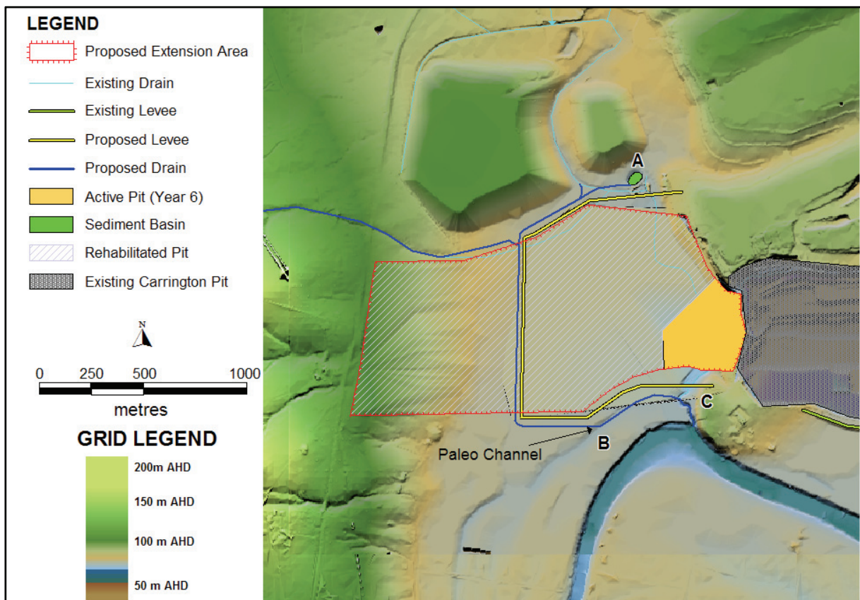
Figure 3.2 Stage 2 Levees and Drainage Channels
