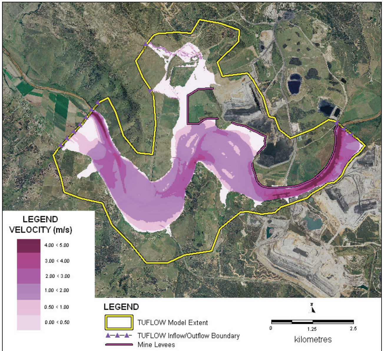
Figure 5.14 Stage 2 Levees and Channel Q100 Flood Depths
