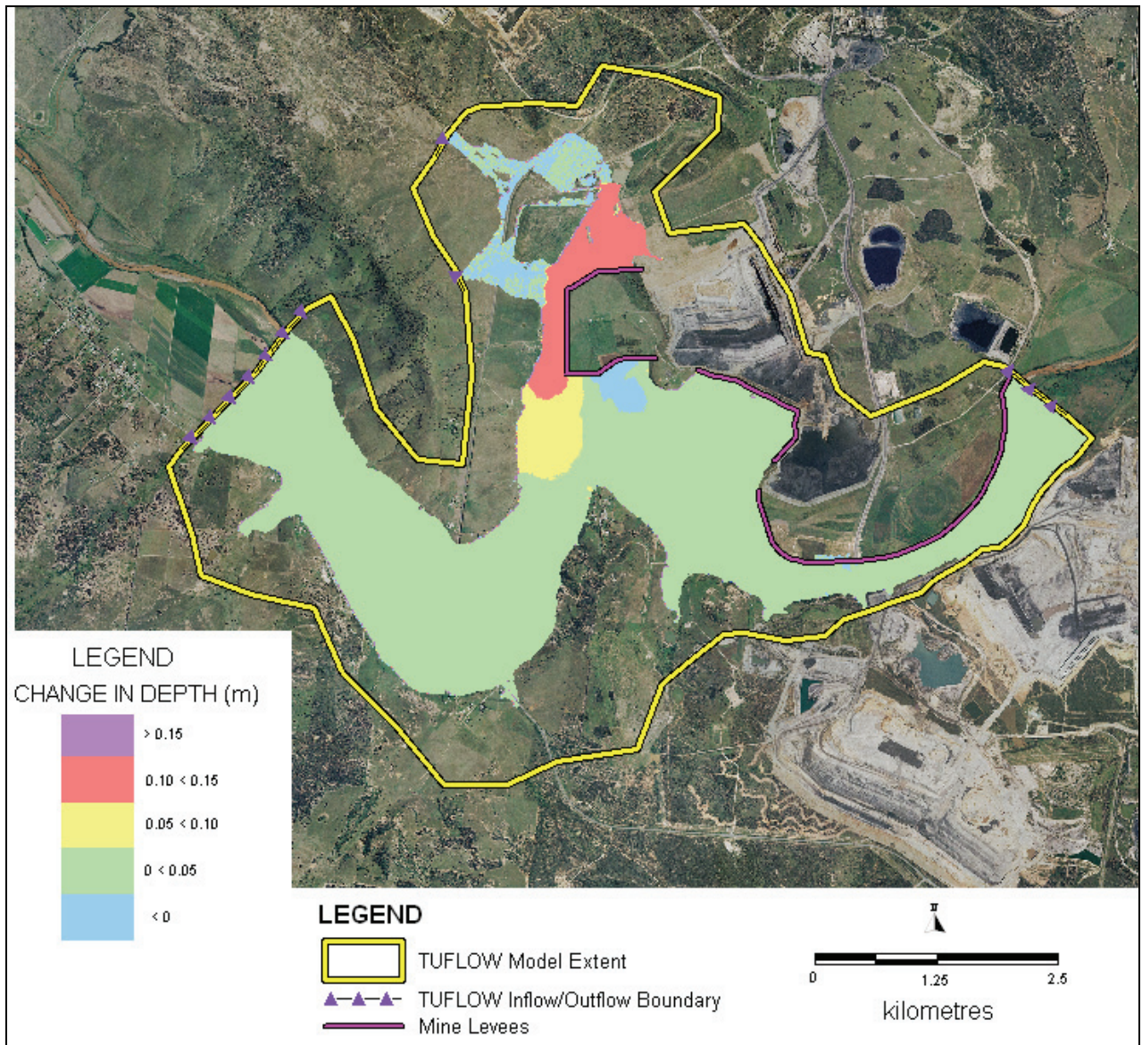
Figure 5.16 Stage 2 Levees Q100 Flood Level Impacts (to existing case)
