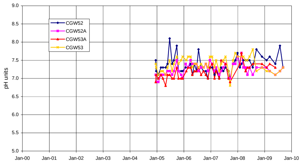
pH at piezometers CGW52, 52A, 53, 53A
