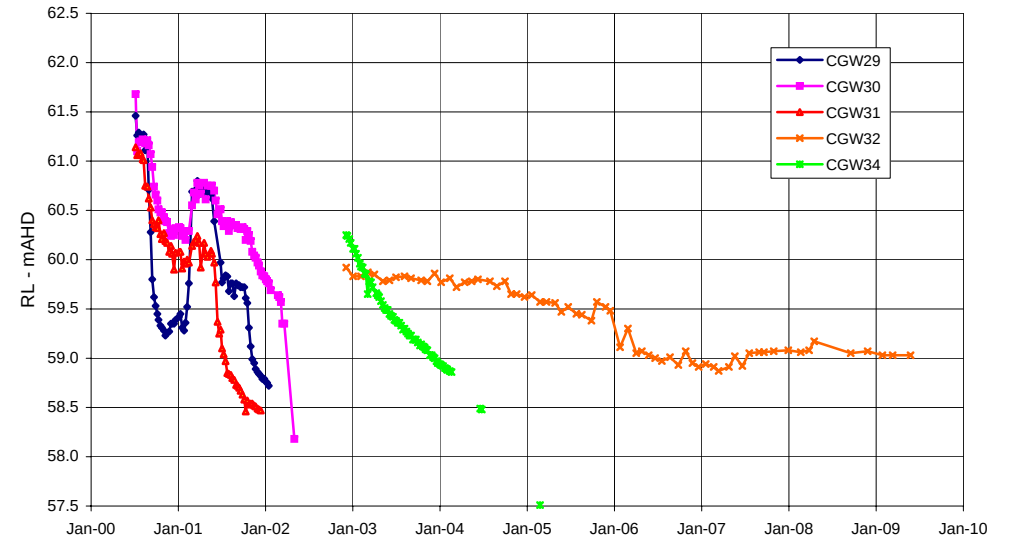
Piezometers CGW 29, 30, 31, 32, 34 - alluvium
