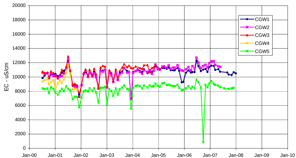
EC at piezometers CGW1, 2, 3, 4, 5
