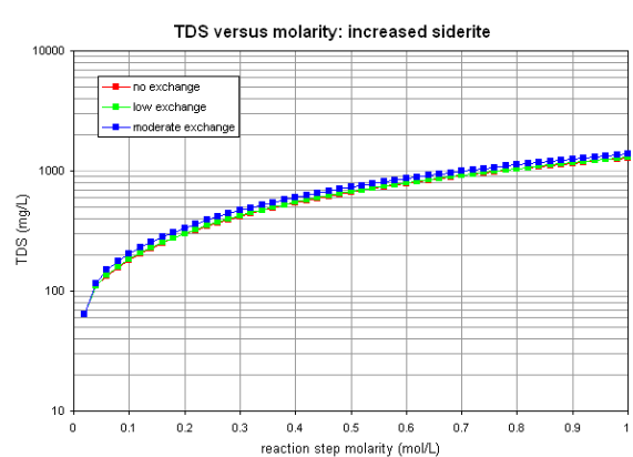
Reaction path model results and comparison to leachate trials
