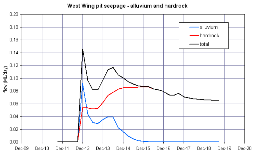
River-alluvium groundwater exchanges and pit seepage
