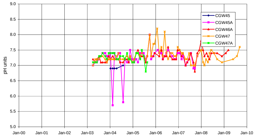
pH at piezometers CGW45, 45A, 46A, 47, 47A
