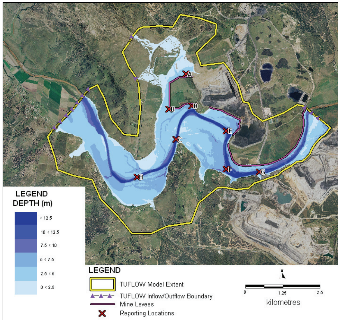
Figure 5.12 Stage 2 Levees and Channel Q10 Flood Depths
