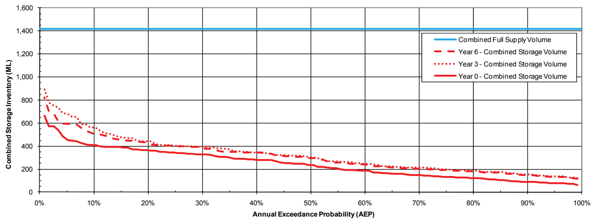
Figure 4.1 Minesite Storage Inventory – Annual Exceedance Probability (AEP)
