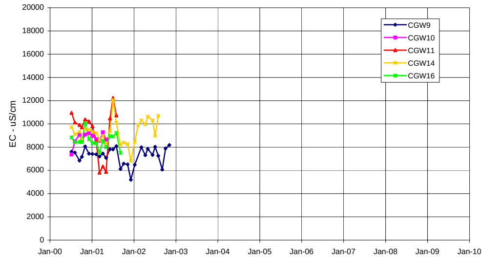
EC at piezometers CGW9, 10, 11, 14,16
