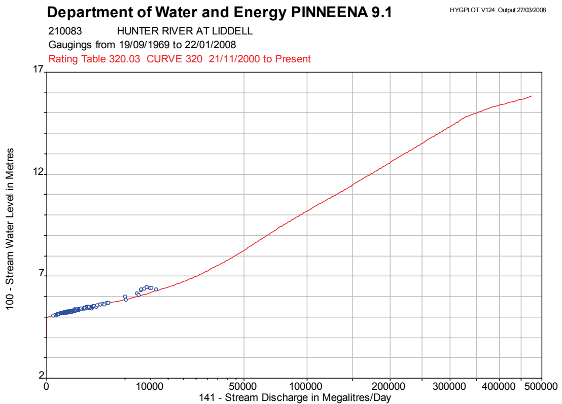
Figure B.7.1 Available Rating Curve, Hunter River at Liddell (210083)
