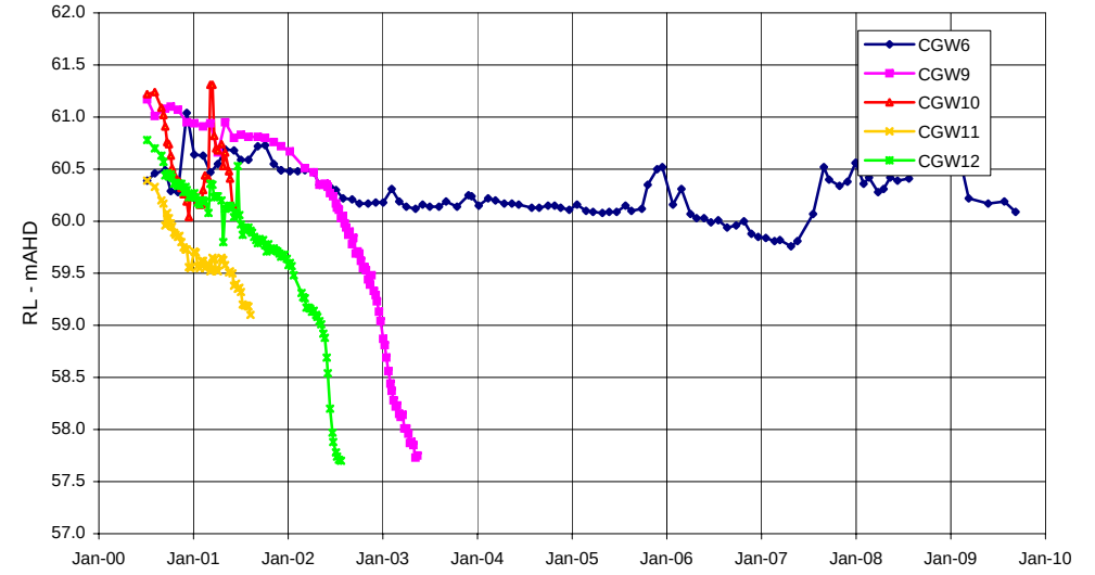
Piezometers CGW6, 9, 10, 11, 12 - alluvium
