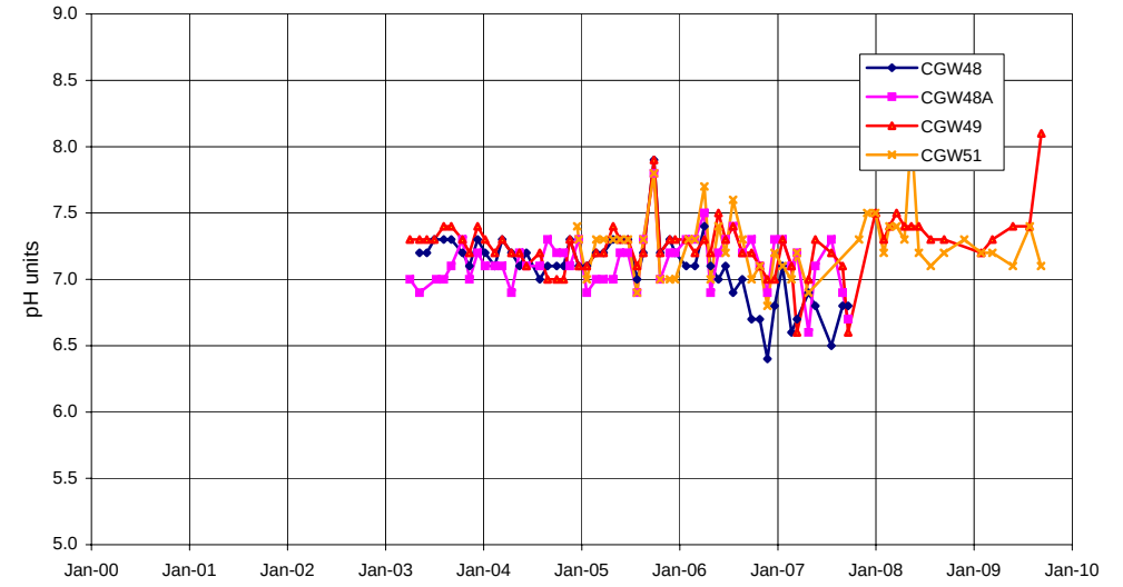
pH at piezometers CGW48, 48A, 49, 51
