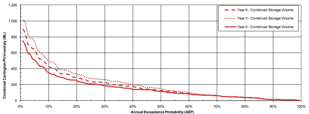
Figure 4.2 Carrington Pit Inventory – Annual Exceedance Probability (AEP)
