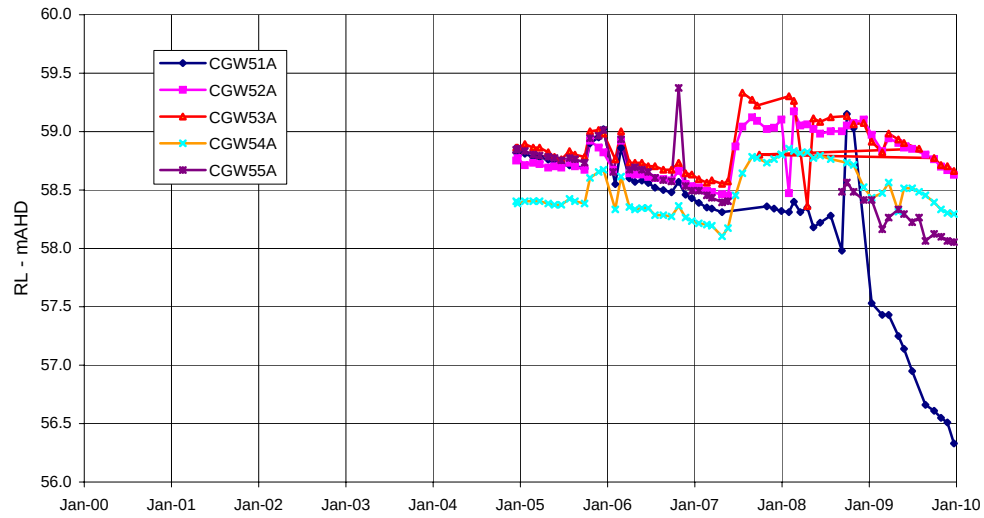
Piezometers CGW51A, 52A, 53A, 54A, 55A - alluvium
