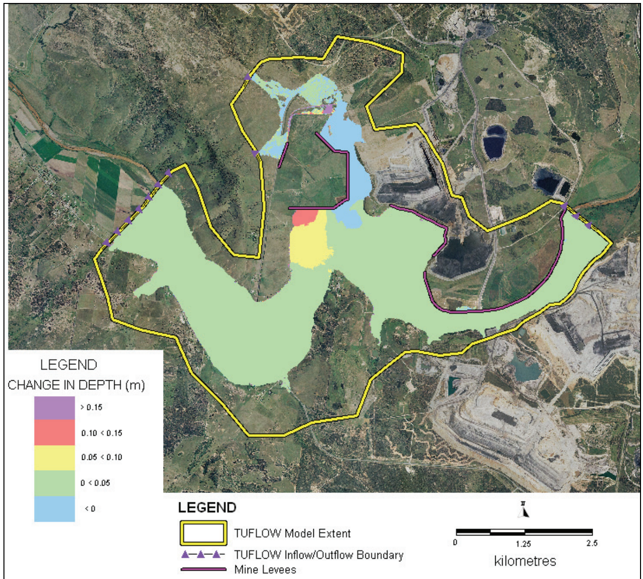
Figure 5.10 Stage 1 Levees Q100 Flood Level Impacts (compared to existing case)
