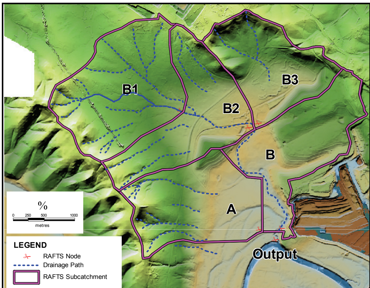
Figure B.7.6 Unnamed Tributary RAFTS Subcatchments
