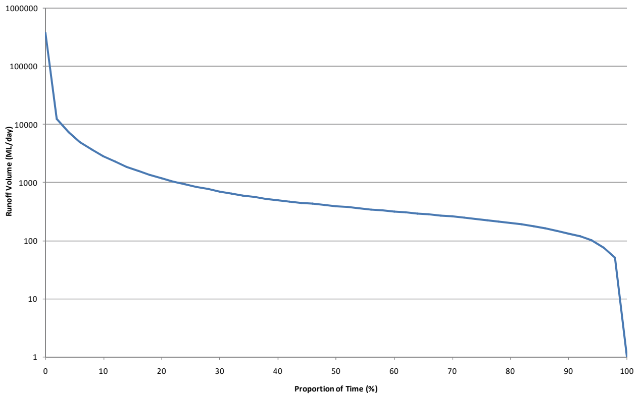
Figure 2.4 Derived Flow-Duration Relationship for the Hunter River at Liddell (1949-2009)
