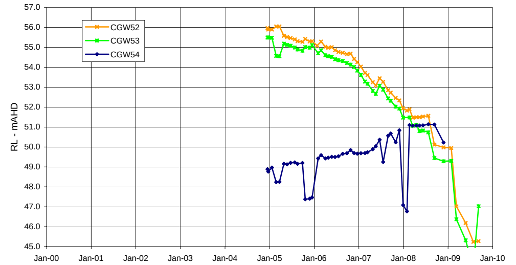
Piezometers CGW52, 53, 54 - Permian
