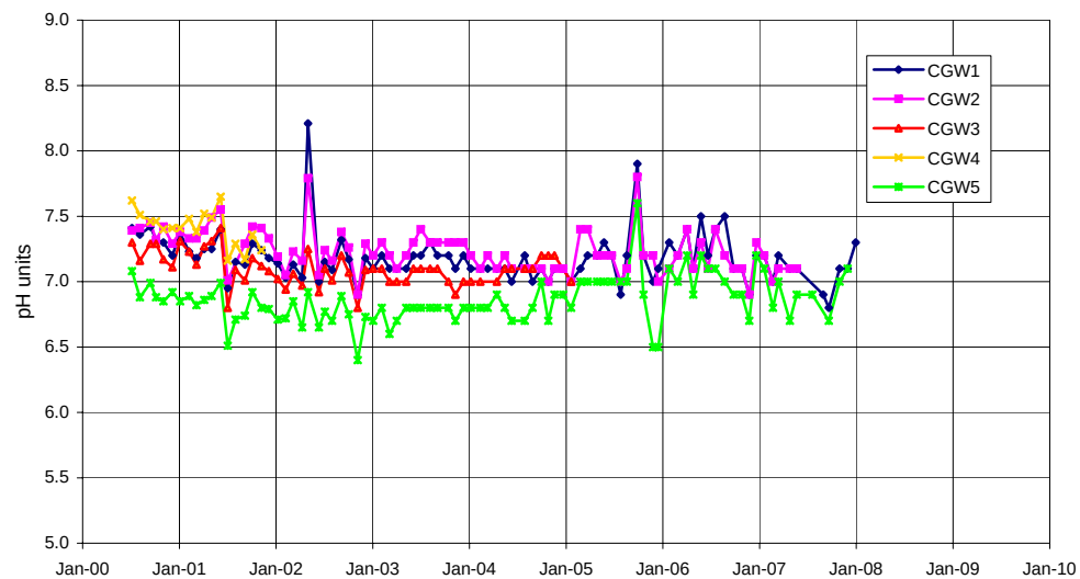
pH at piezometers CGW1, 2, 3, 4, 5
