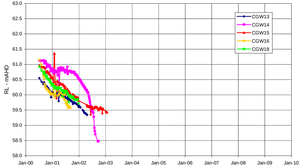
Piezometers CGW13, 14, 15, 16, 18 - alluvium
