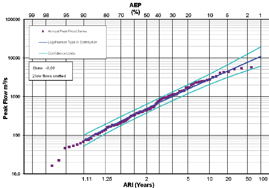
Figure B.7.4 Flood Frequency Distribution, Hunter River at Singleton (210001)
