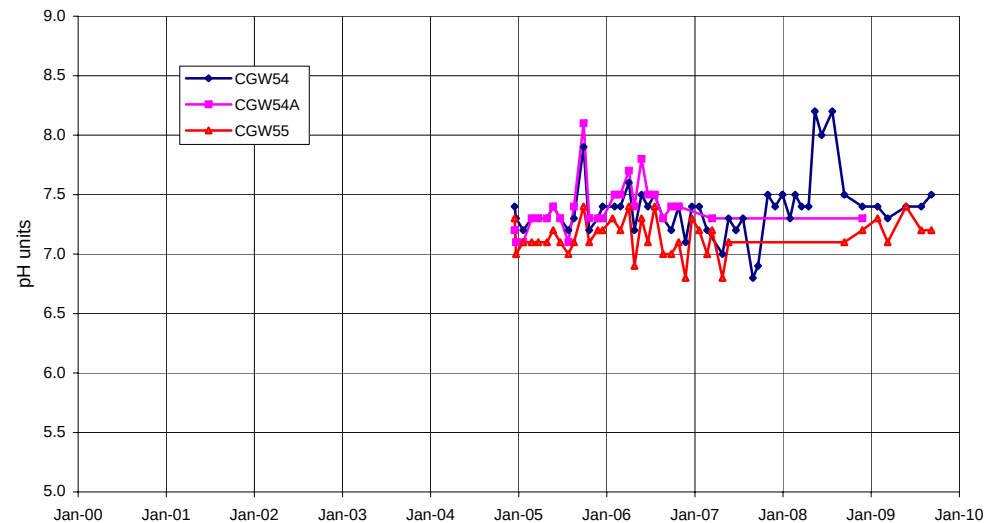
pH at piezometers CGW54, 54A, 55
