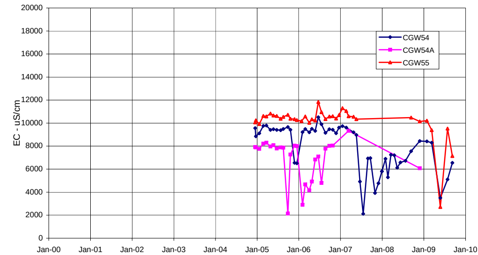
EC at piezometers CGW54, 54A, 55
