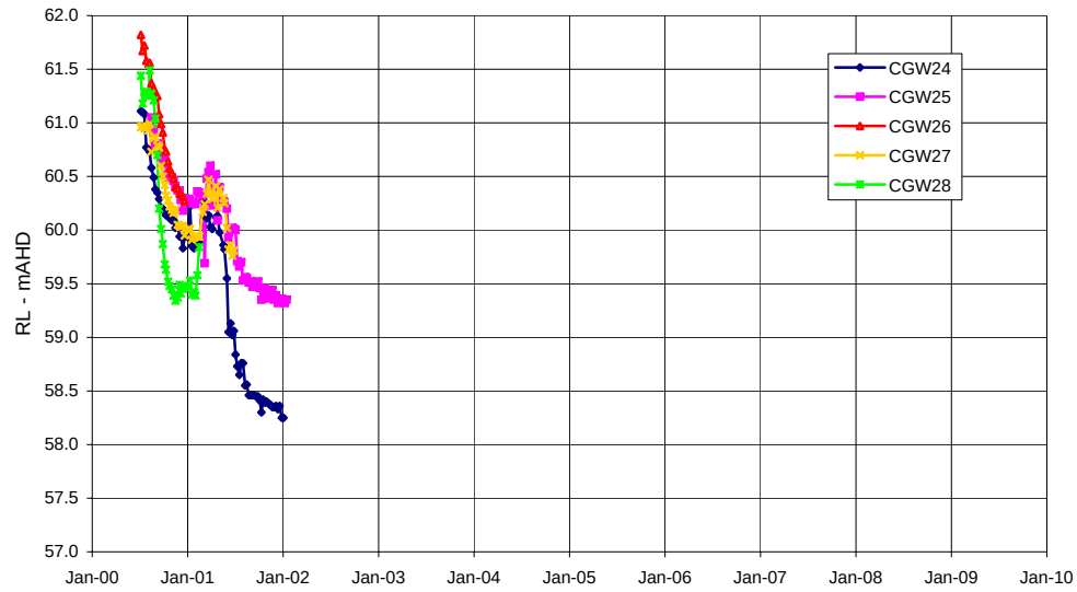
Piezometers CGW 24, 25, 26, 27, 28 - alluvium
