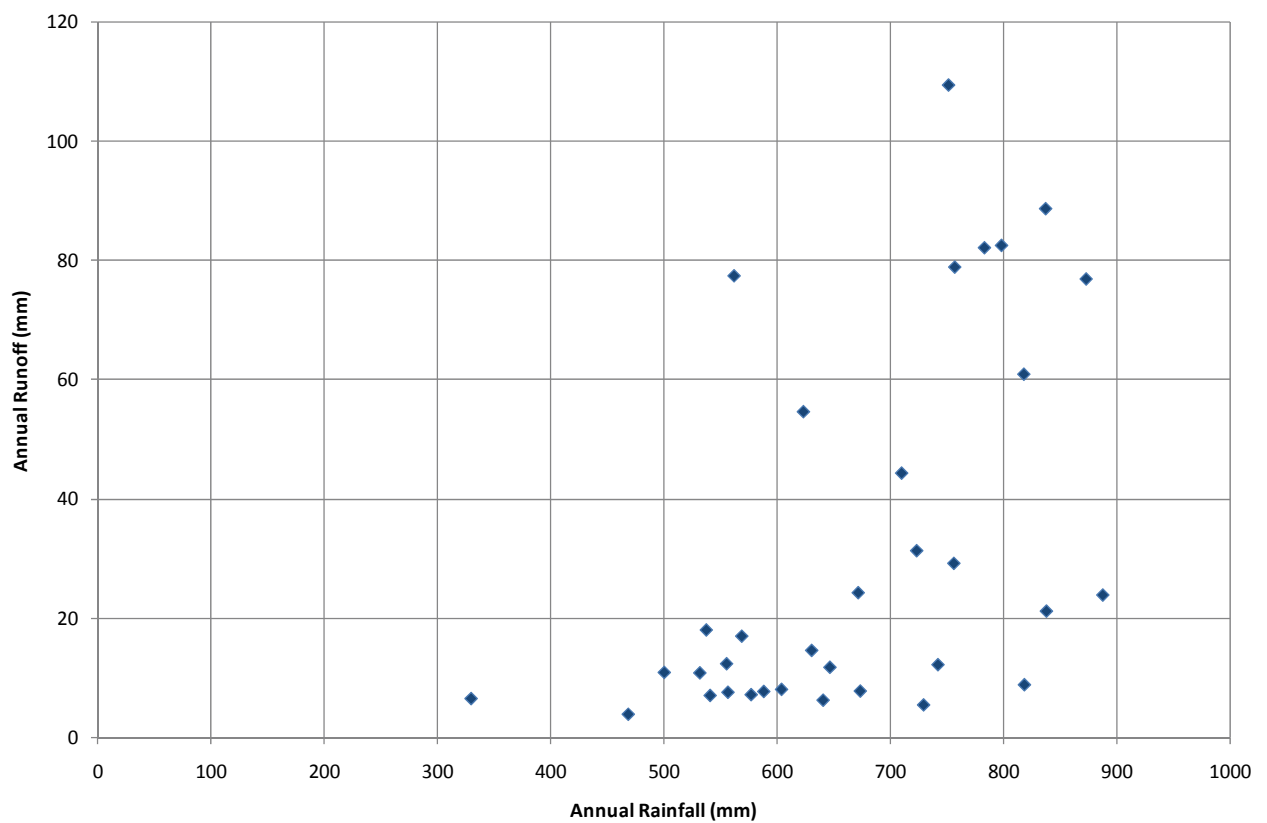
Figure 2.5 Annual Runoff versus Rainfall for the Hunter River at Liddell Gauging Station
