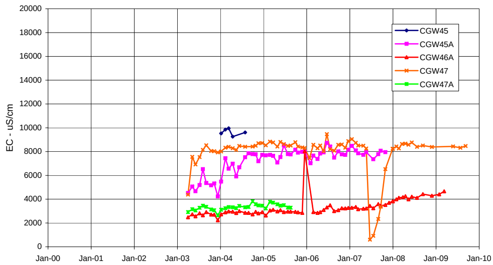
EC at piezometers CGW45, 45A, 46A, 47, 47A
