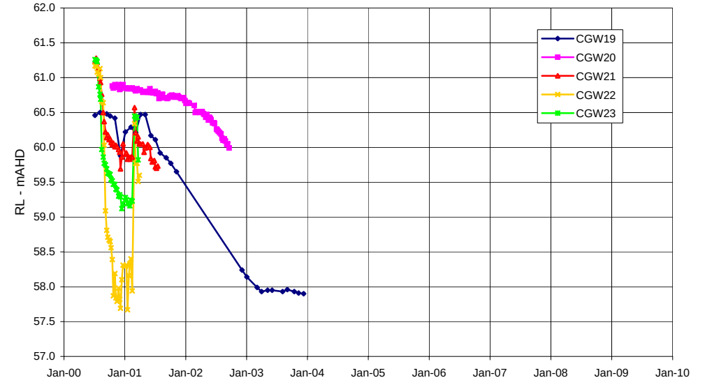
Piezometers CGW19, 20, 21, 22, 23 - alluvium
