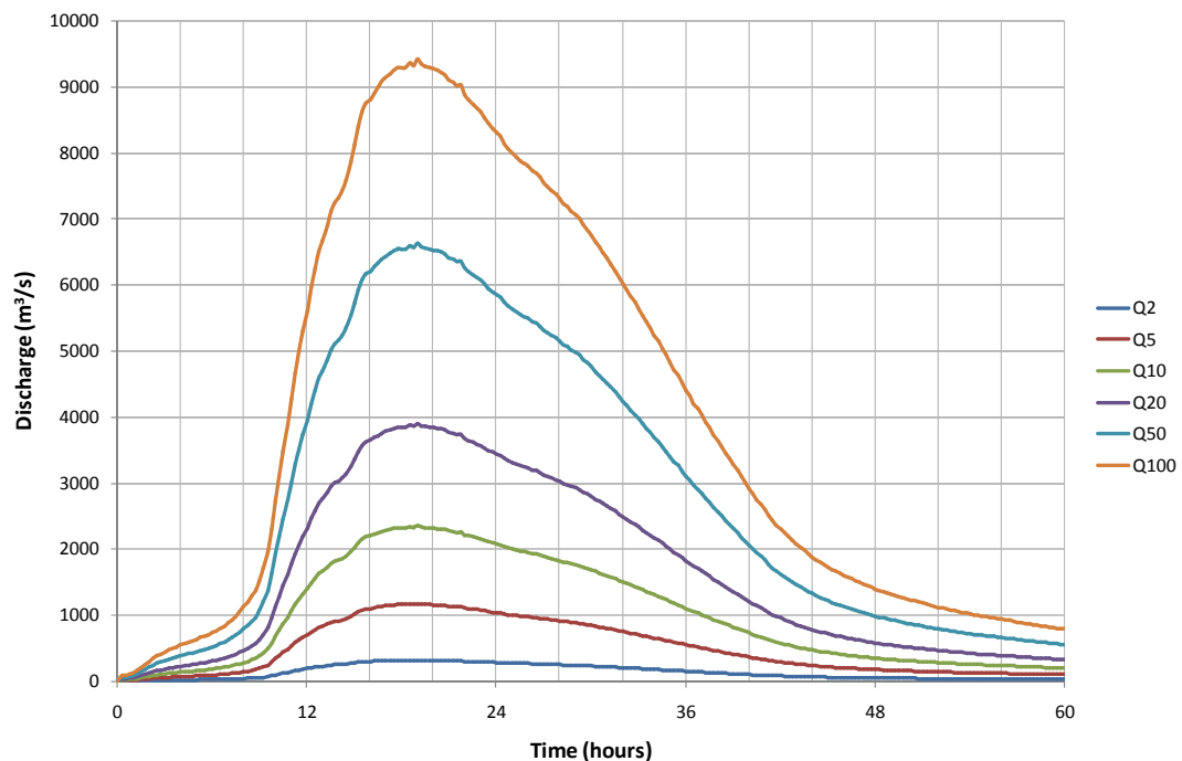
Figure B.7.5 Adopted Hydrographs, Hunter River at Liddell
