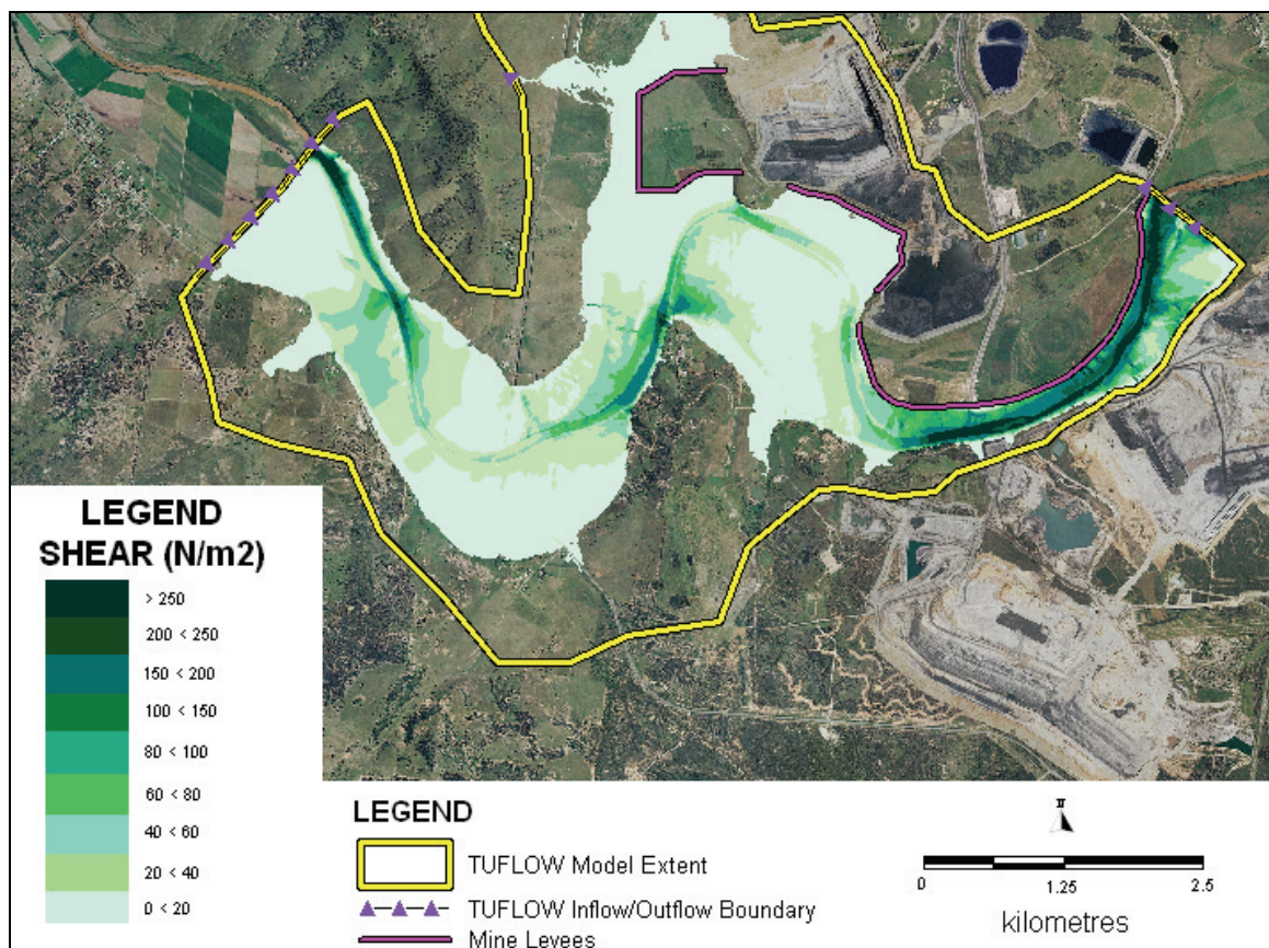
Figure 5.18 Hunter River Bed Shear, 100 Year ARI Flood
