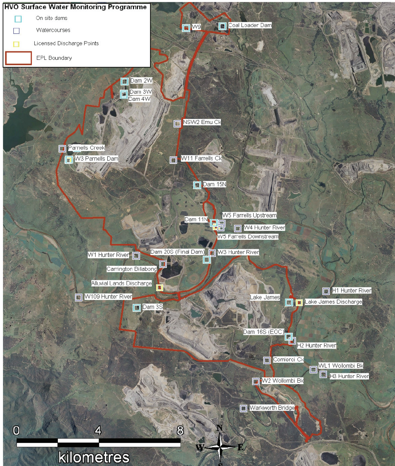
Figure 2.6 HVO Surface Water Monitoring Network
