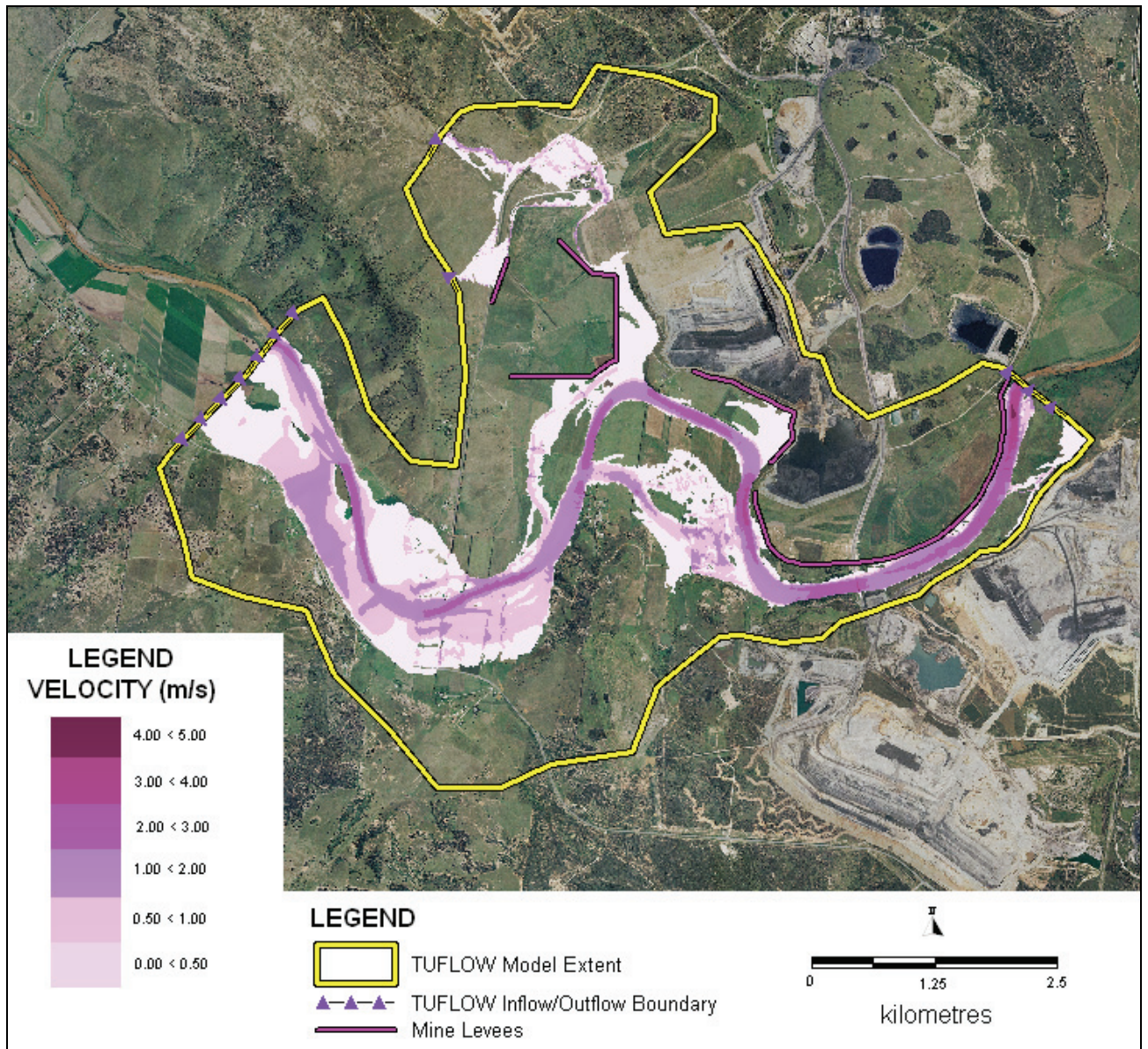
Figure 5.7 Stage 1 Levees Q10 Flood Velocities
