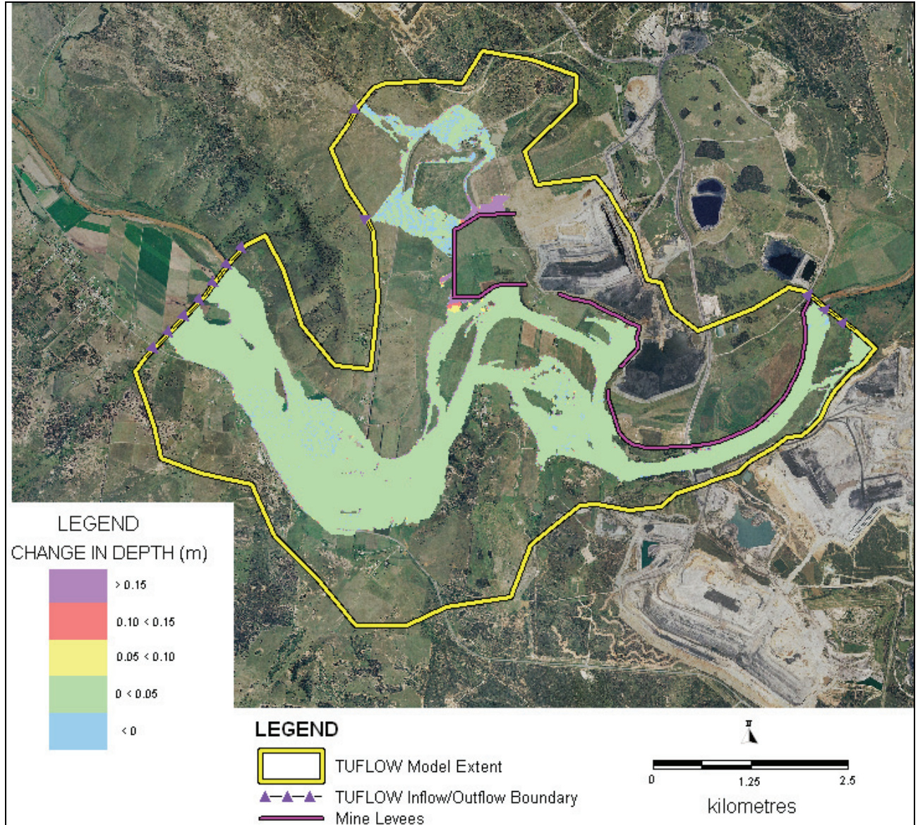
Figure 5.15 Stage 2 Levees Q10 Flood Level Impacts (compared to existing case)
