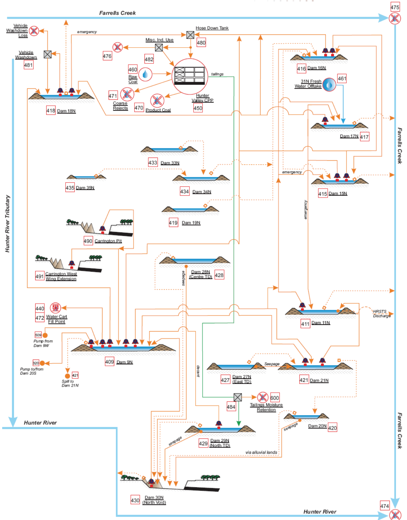
Figure 2.7 Minesite Water Management System Schematic
