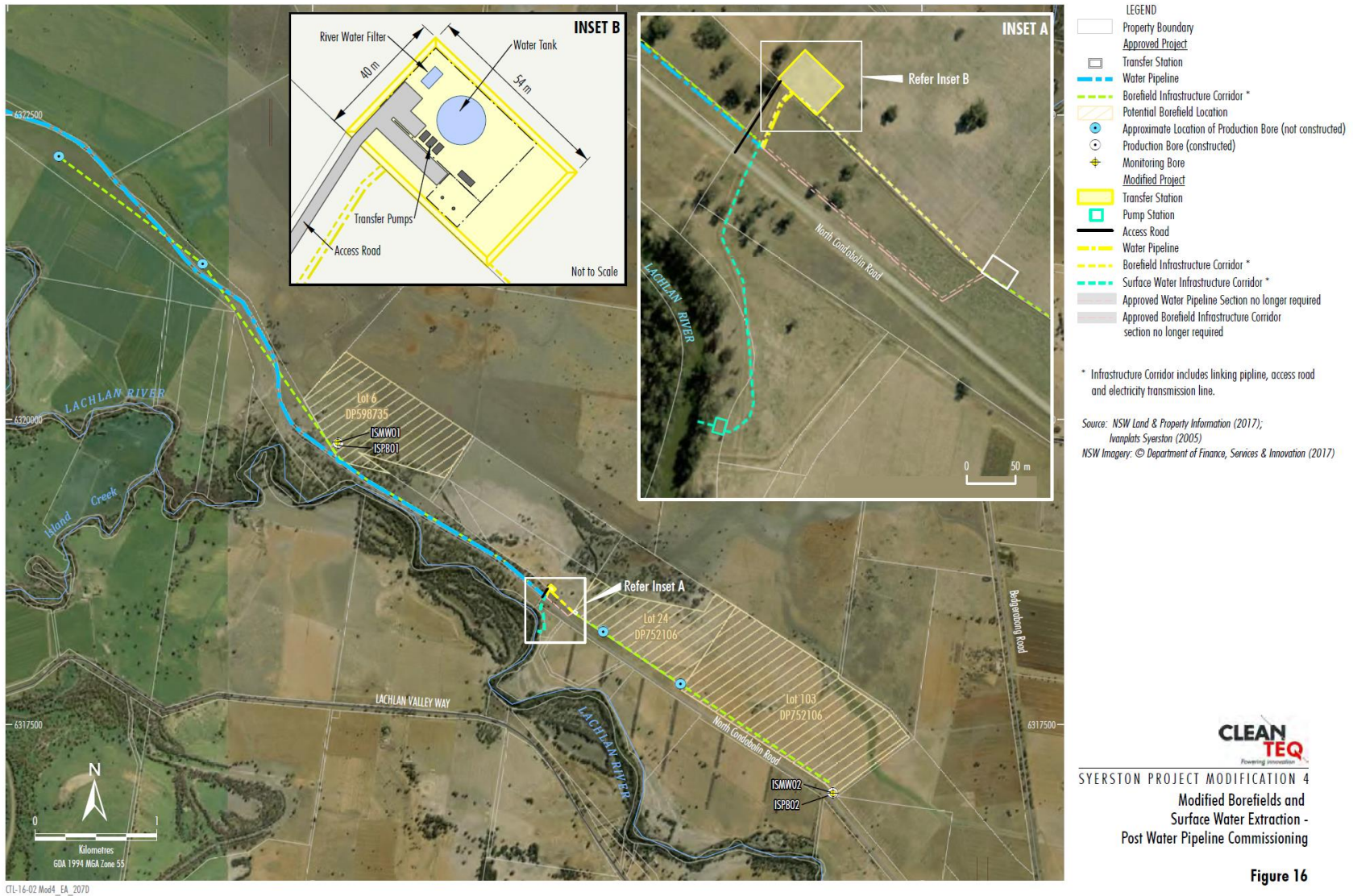
Figure 9: Borefields Layout
