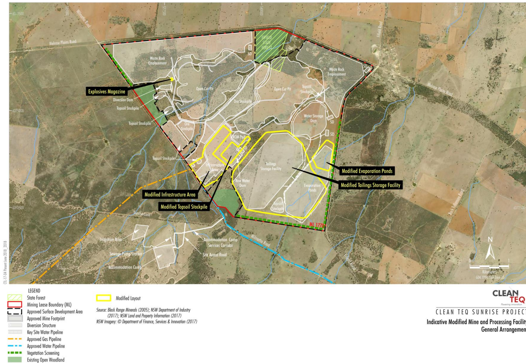
Figure 2: Mine and Processing Facility – General Layout
