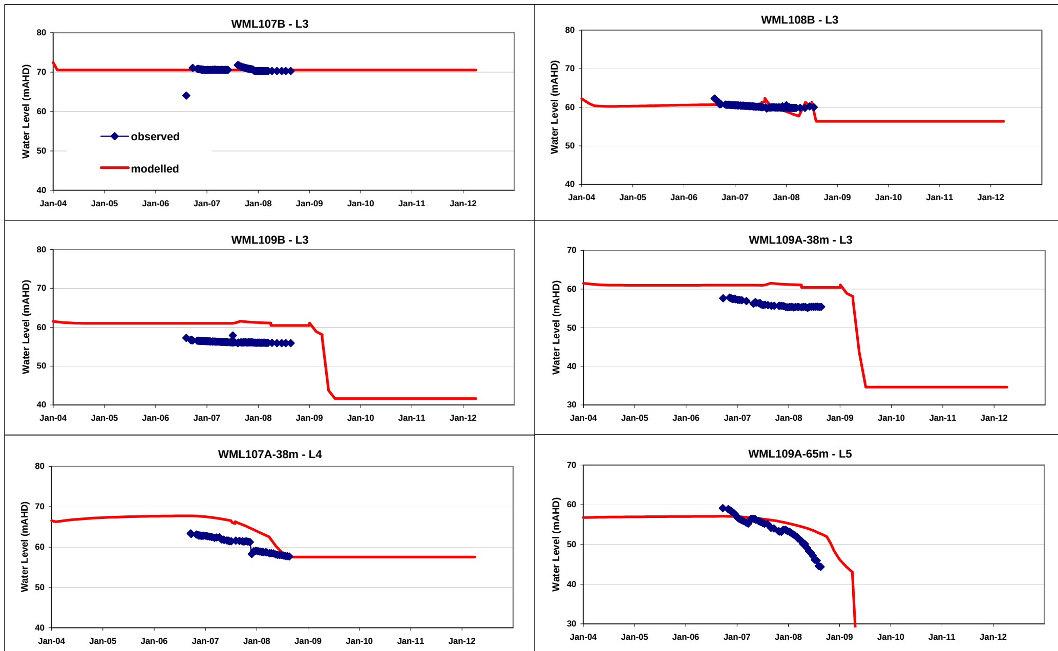
Layers 3 to 4 Modelled vs Observed - Lemington 7-9 Seams (L3), Lemington 11 (L4), Lemington 12 (L5) Water Levels
