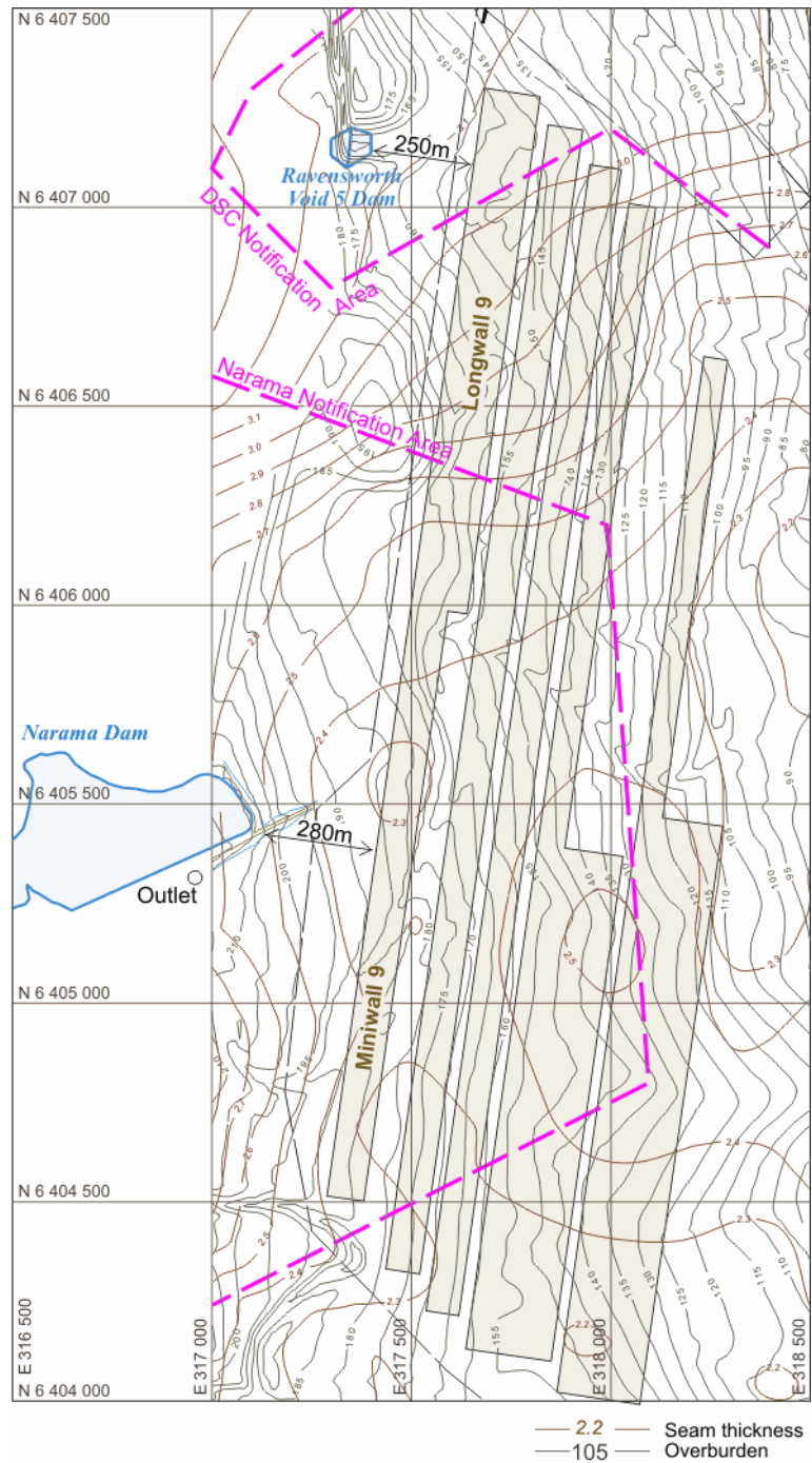
Figure 1 Site plan showing location of Narama Dam and Ravensworth Void 5 Dam.
