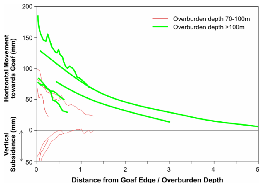
Figure 3 Examples of vertical and horizontal subsidence movements measured at Ashton and elsewhere.
