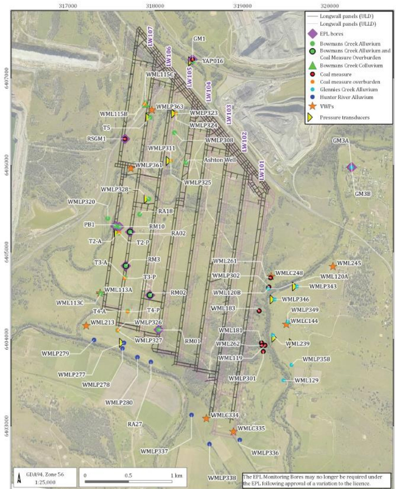
Figure 8 Groundwater Level Baseline and Trigger Level Monitoring Bores
