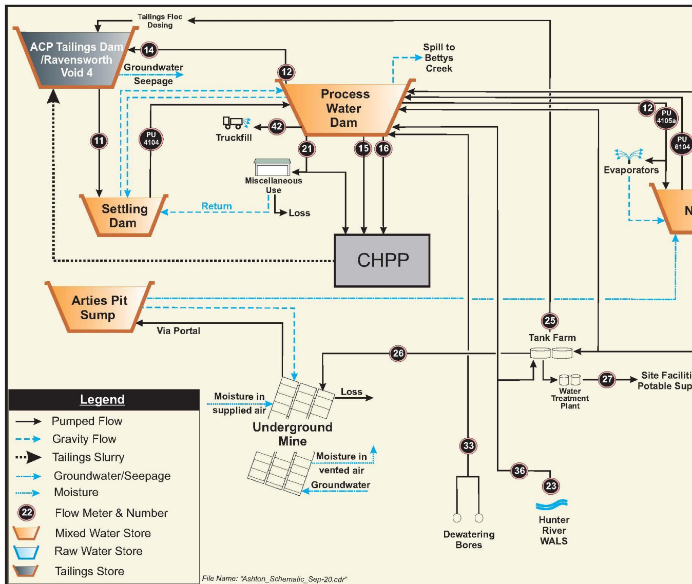
Figure 3. The model operates on a sub-daily time-step and has been setup to simulate the forward planning period from mid-2019 to the end of December 2030.
