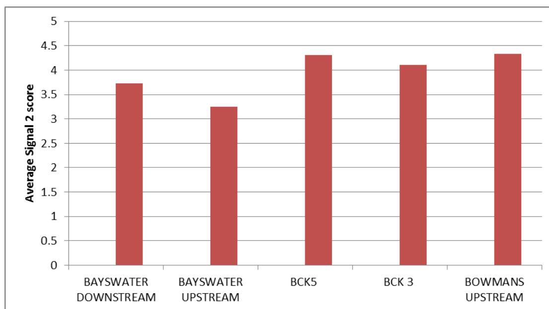
Figure 7: Average SIGNAL 2 Score for sites on Bayswater and Bowmans Creeks
