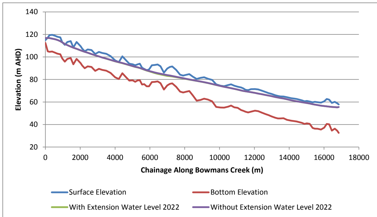
Figure 13. Expected drawdown along the Bowmans Creek alluvium (provided by SKM 2013)
