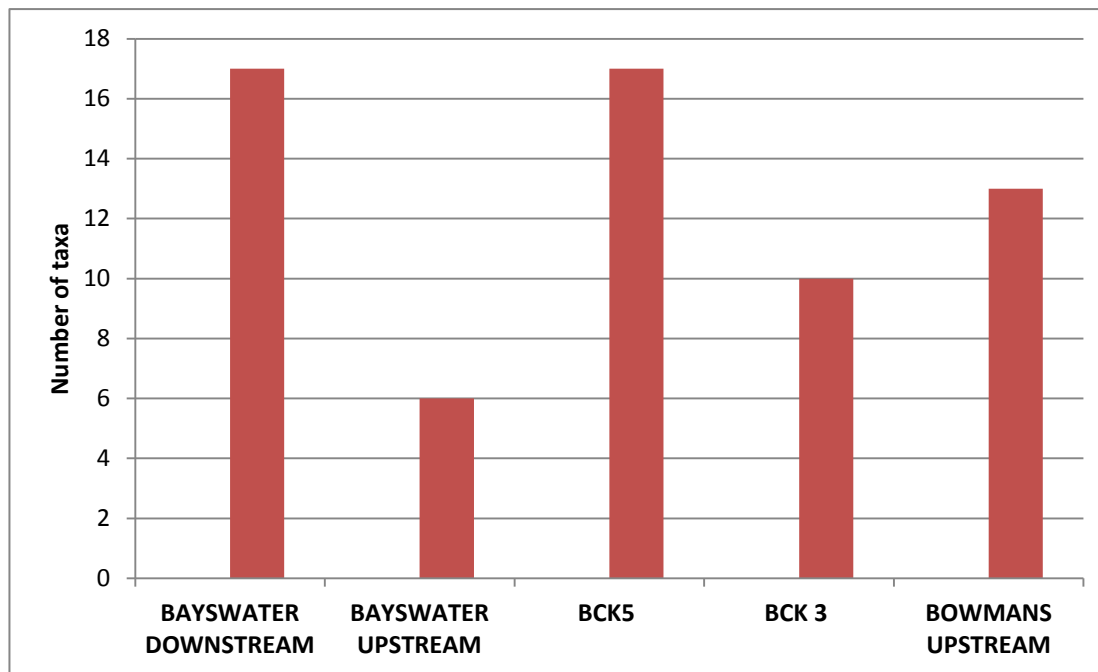
Figure 6: Number of invertebrate taxa per site at Bayswater and Bowmans Creek.
