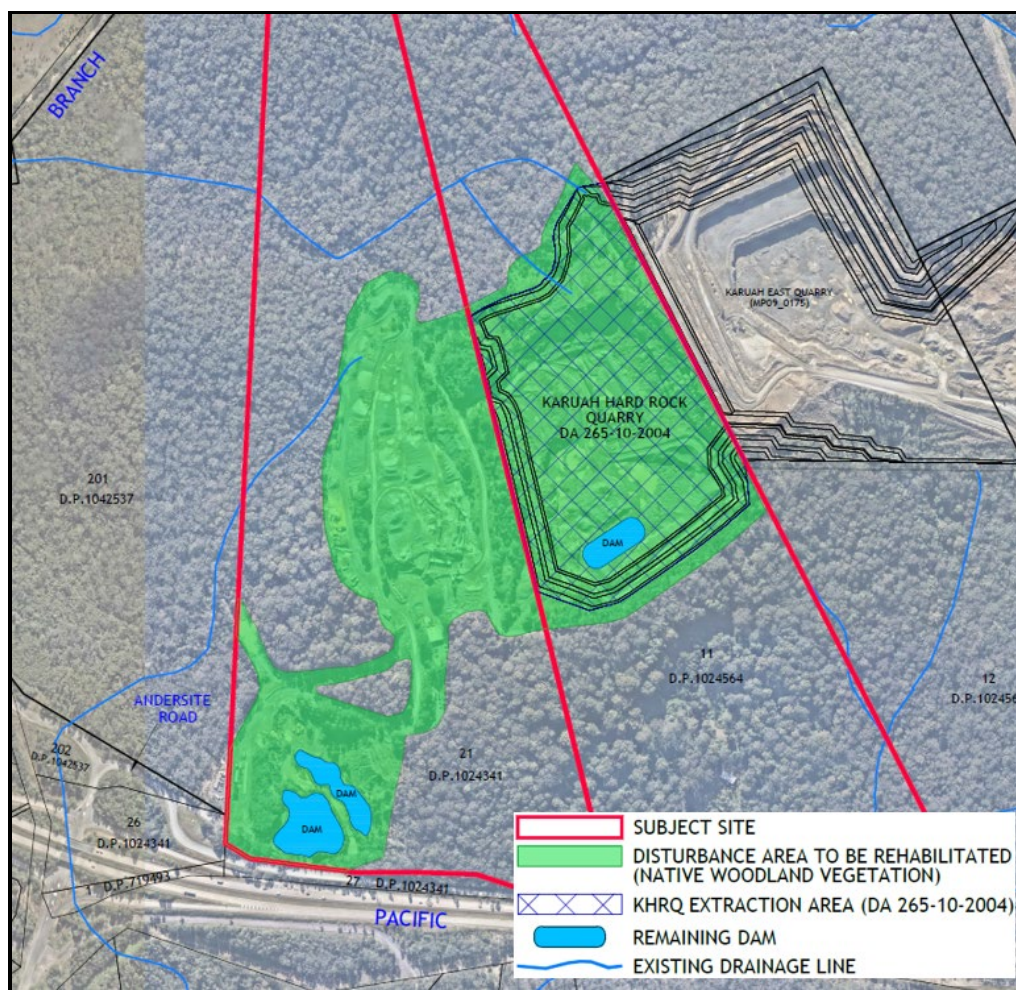
Concept Final Rehabilitation Plan
