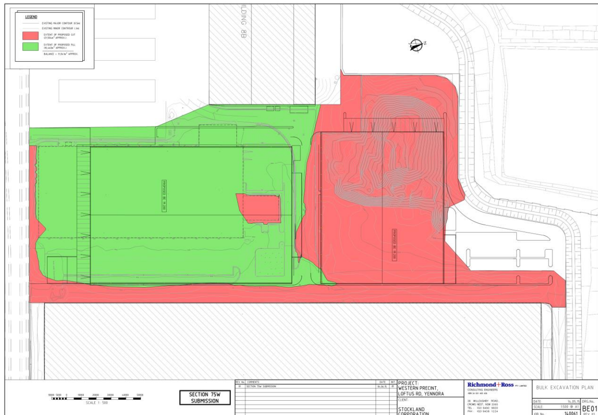
Figure 2 – Bulk Earthworks Plan
