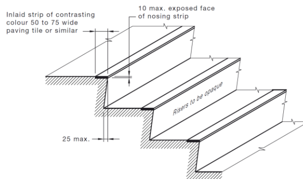
Figure 10: Nosing Details
