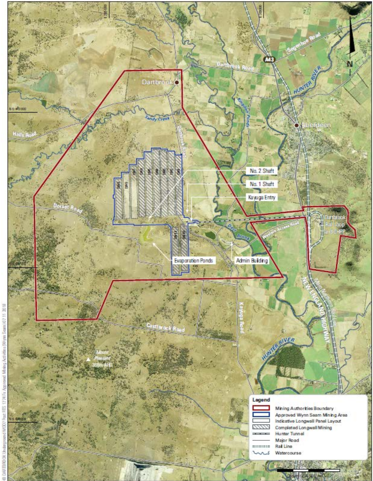
Figure 6: Approved Longwall Mine Plan - Wynn Seam
