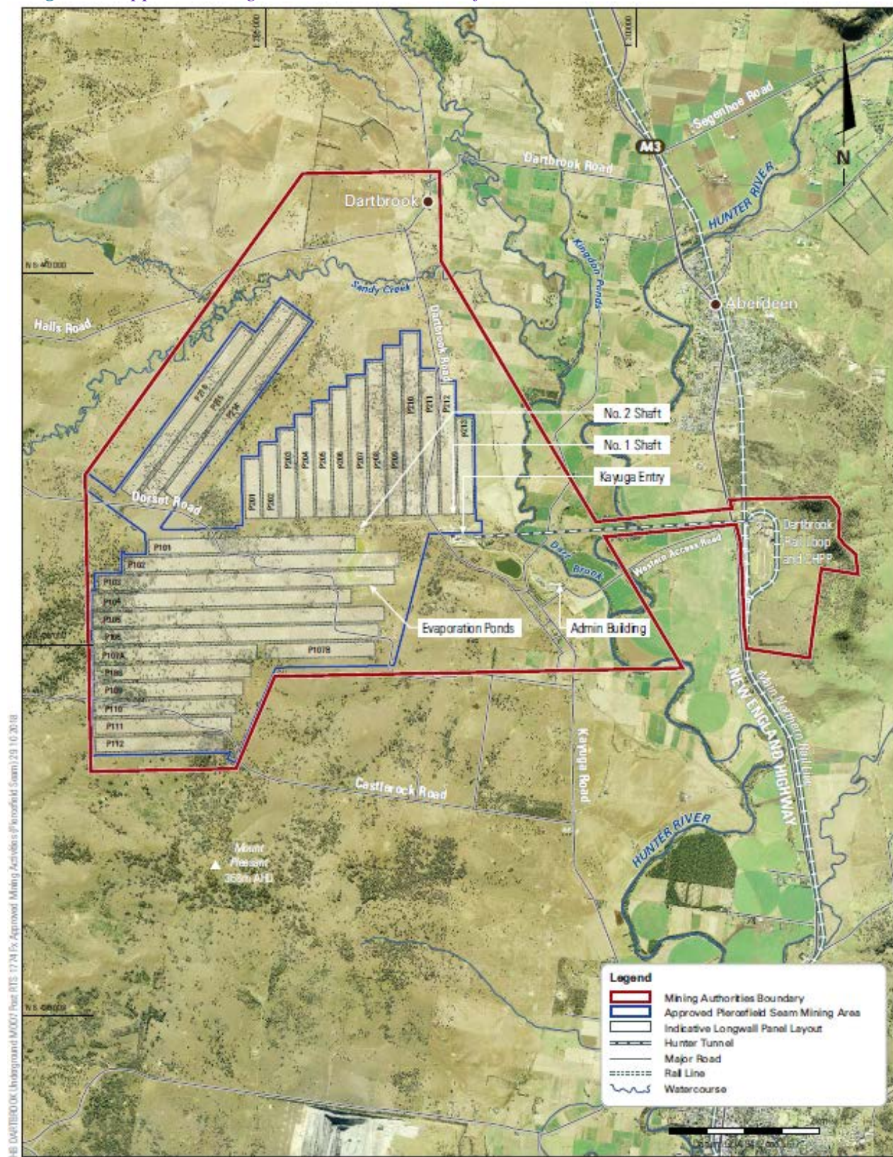
Figure 5: Approved Longwall Mine Plan – Piercefield Seam
