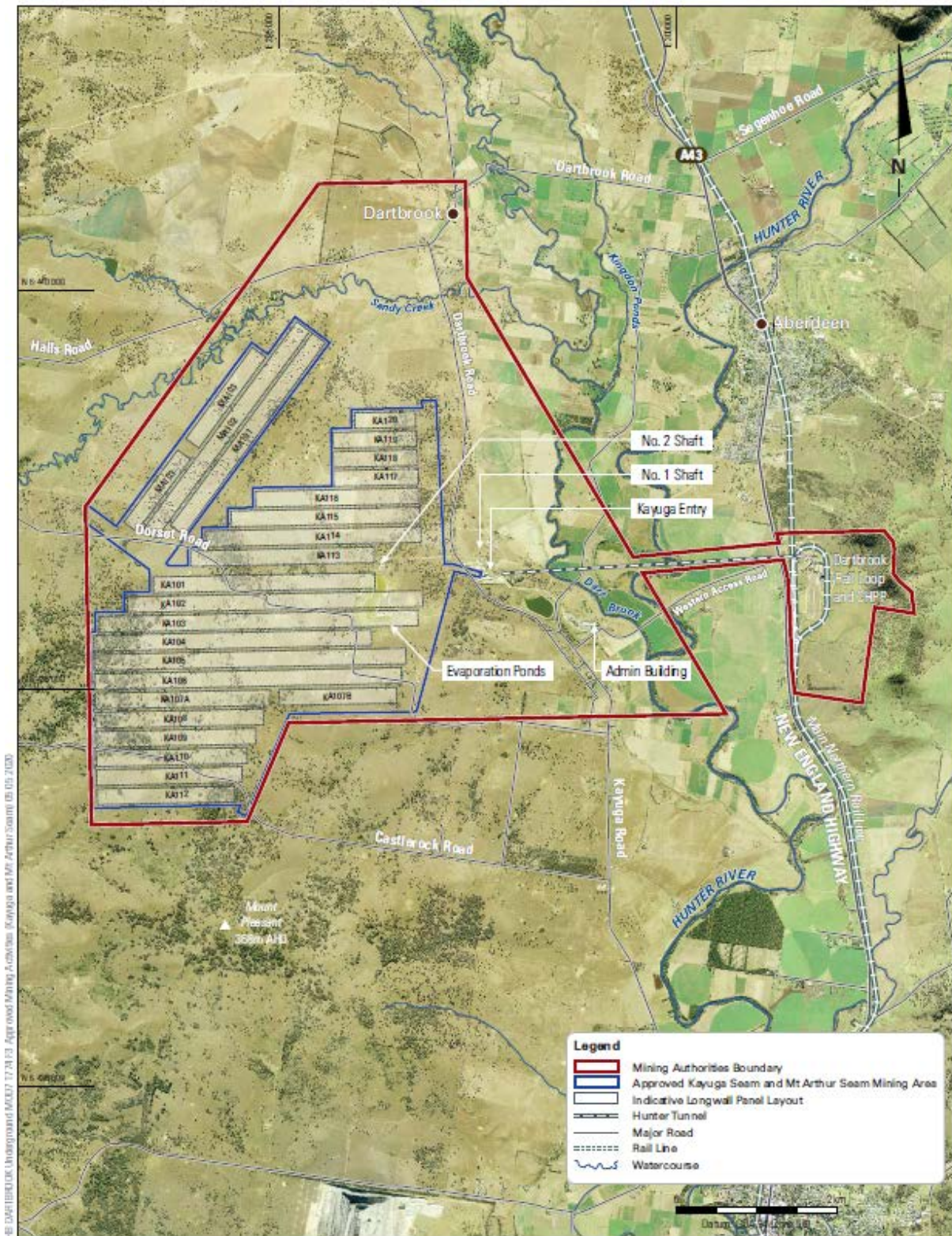
Figure 4: Approved Longwall Mine Plan -Kayuga and Mt Arthur Seams
