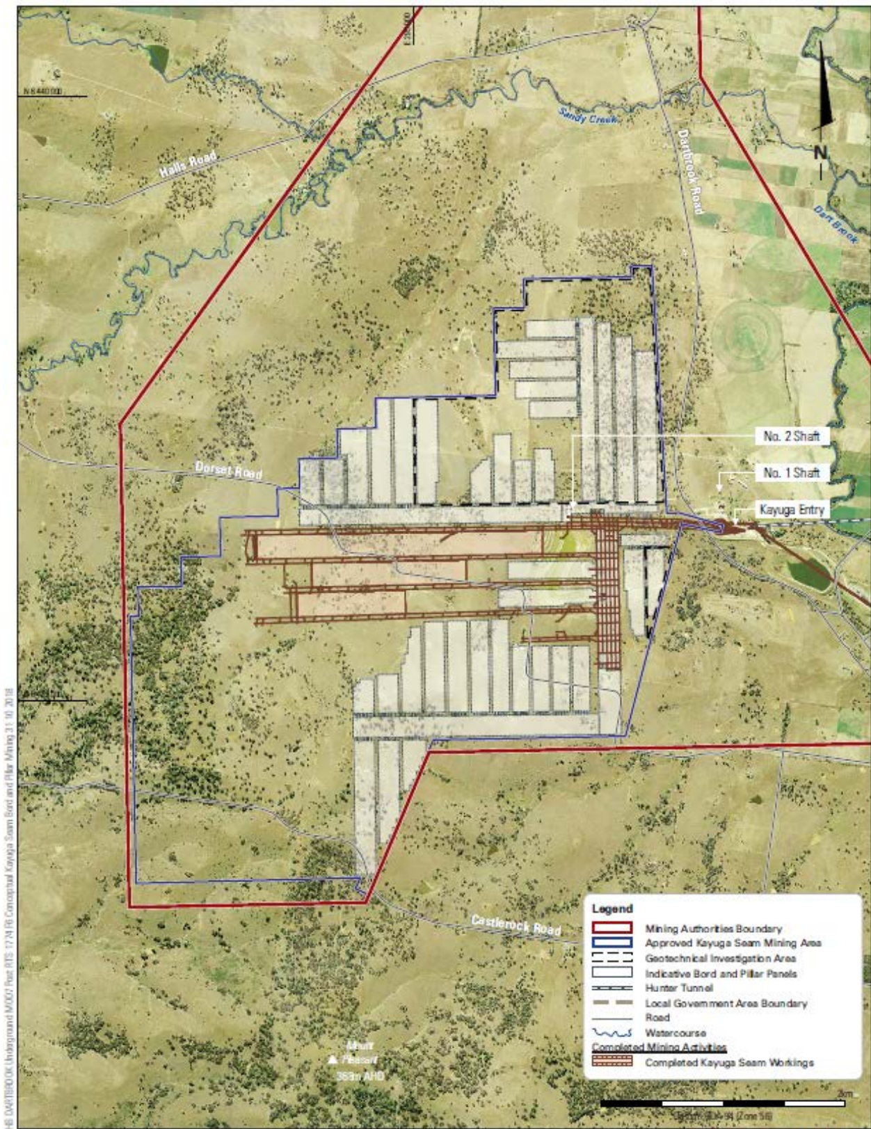
Figure 7: Approved Bord and Pillar Mine Plan -Kayuga Seam
