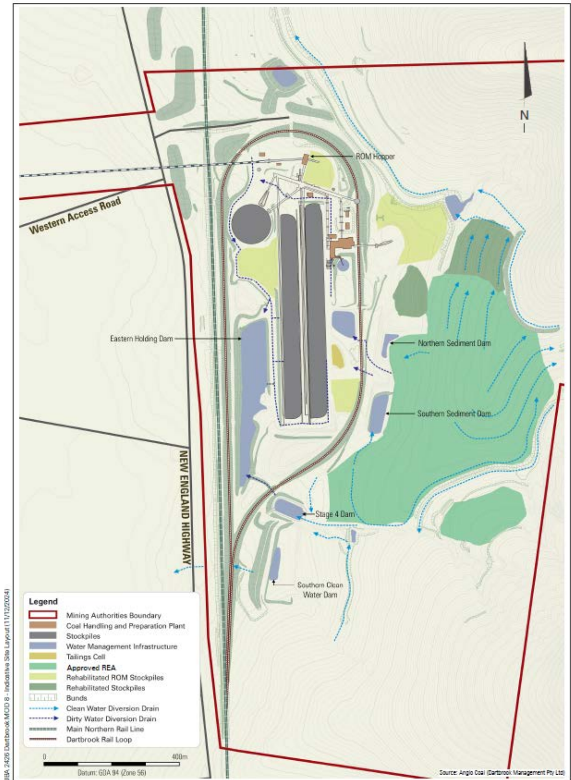
Figure 2: Existing East Site Infrastructure (Figure I of Hansen Bailey Response to Contentions)
