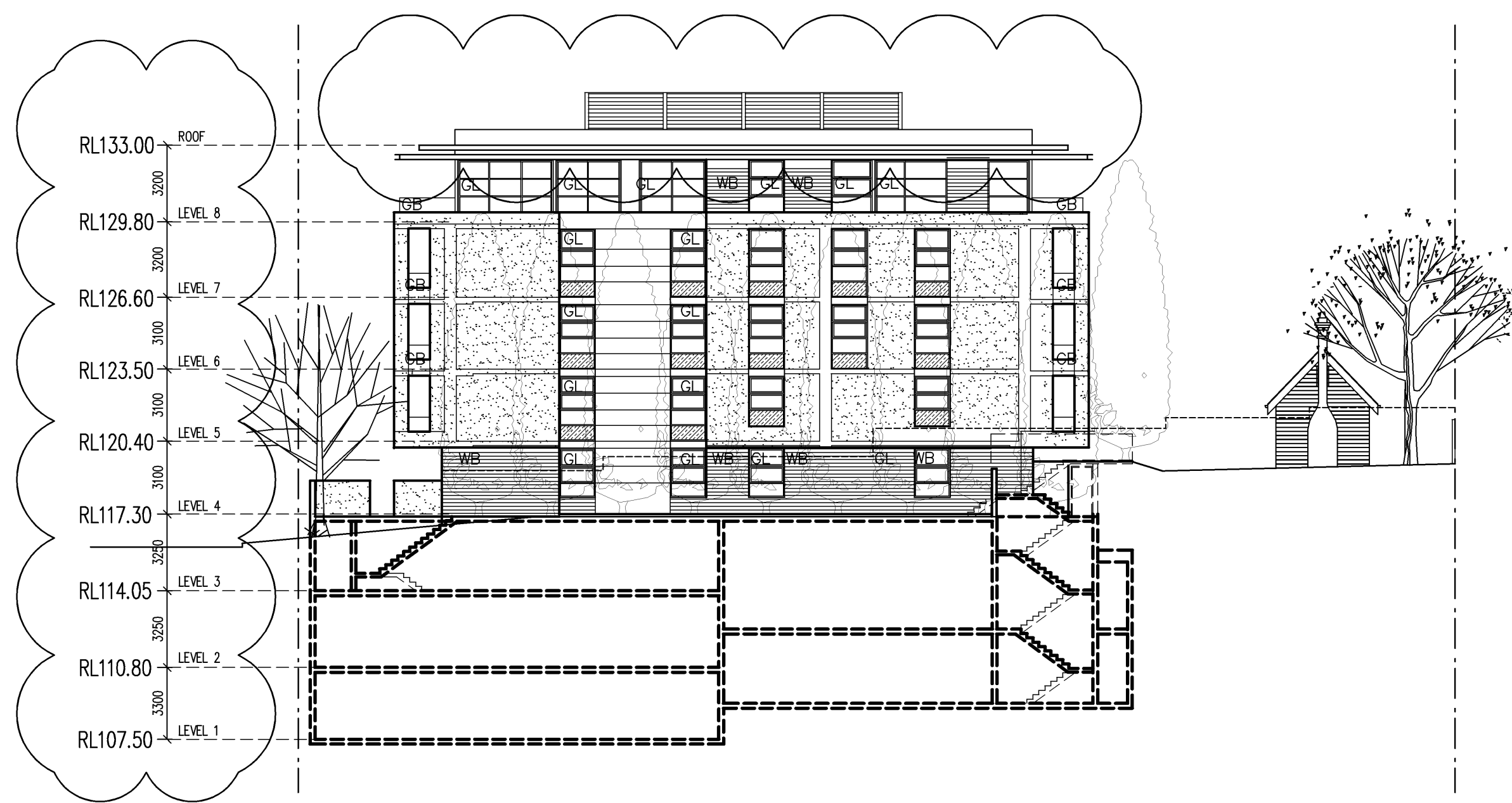
EAST ELEVATION MCINTYRE BUILDING
