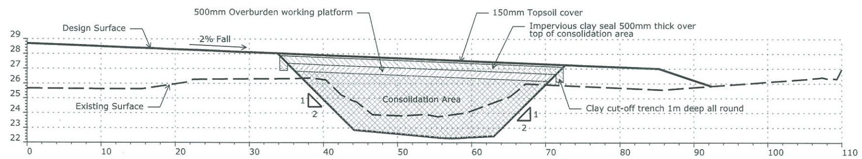
Section A 1:500 (Hor) 1:250 (Ver)
