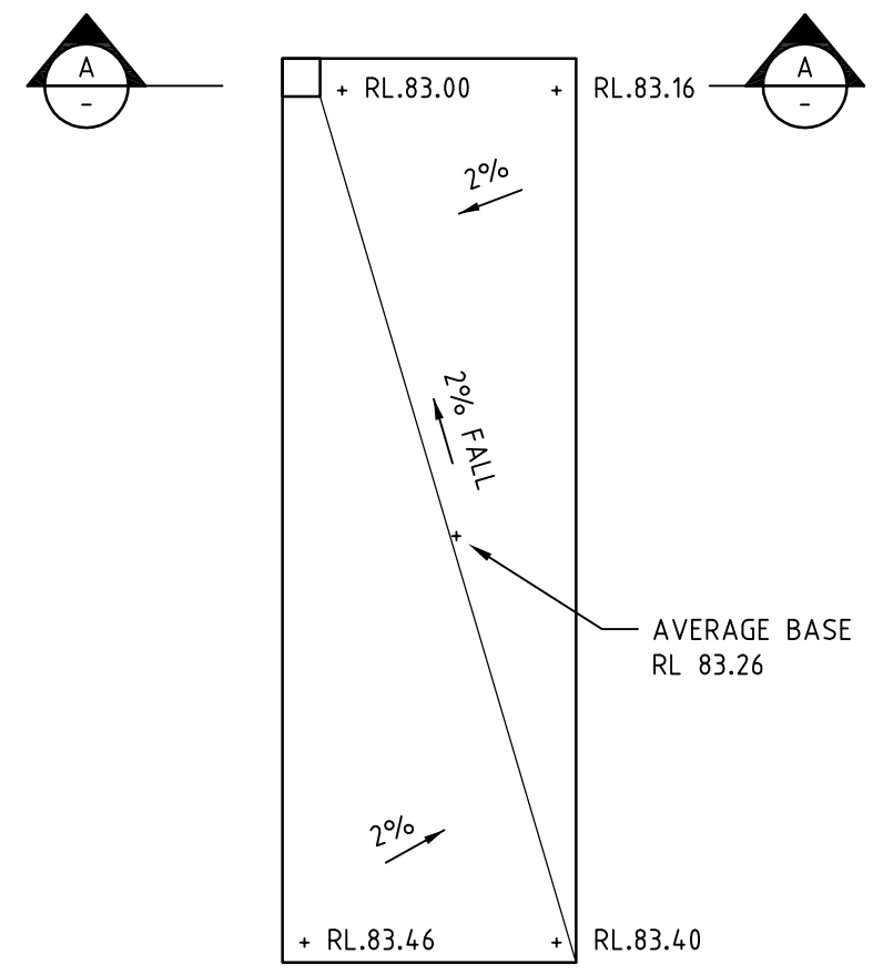
OSD BASE PLAN SCALE 1:200
